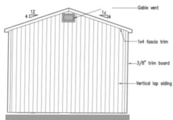
Exterior Elevation
