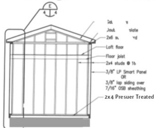
Wall Framing Elevation
