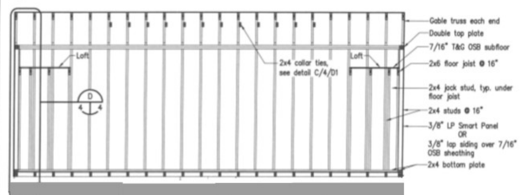
Wall Framing Elevation
