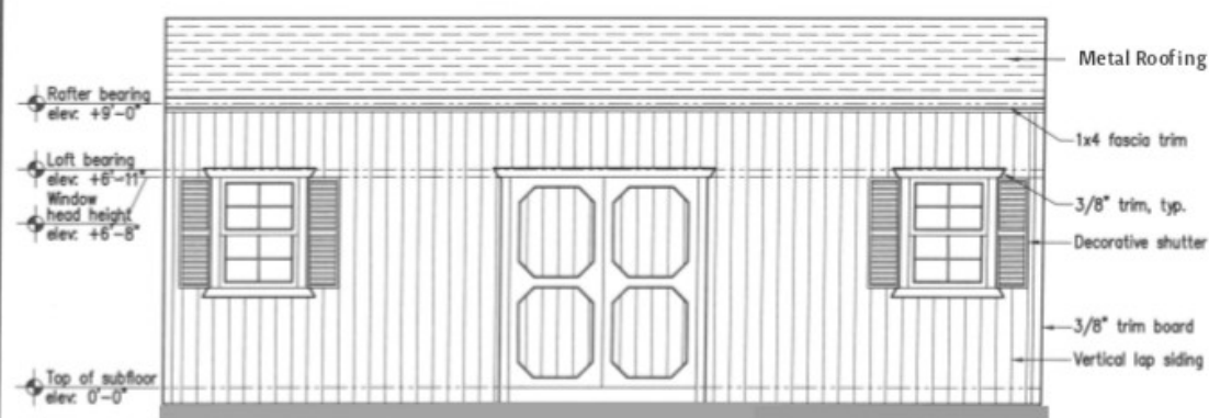
Exterior Elevation
