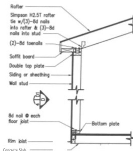
Wall Section
