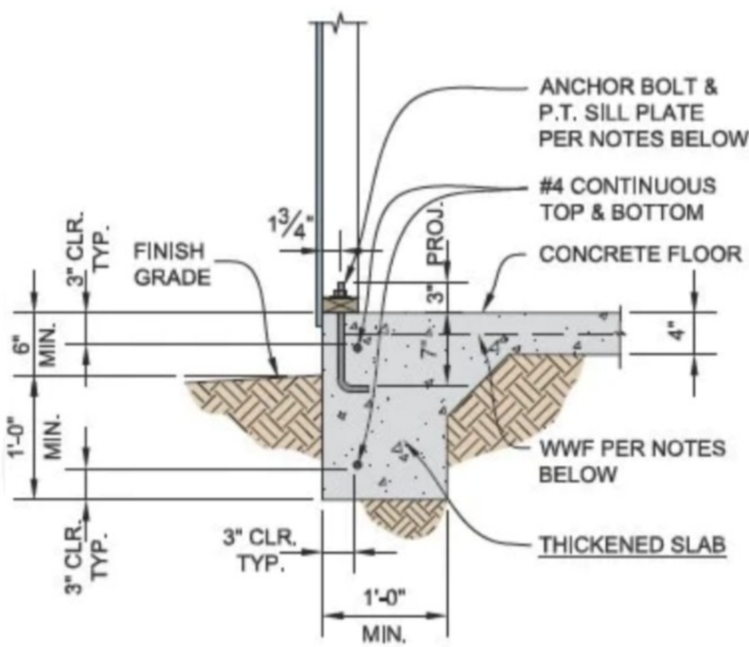
Monolithic Foundation
