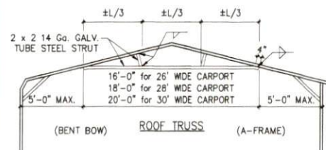
1 2 TYPICAL BOW SECTION
