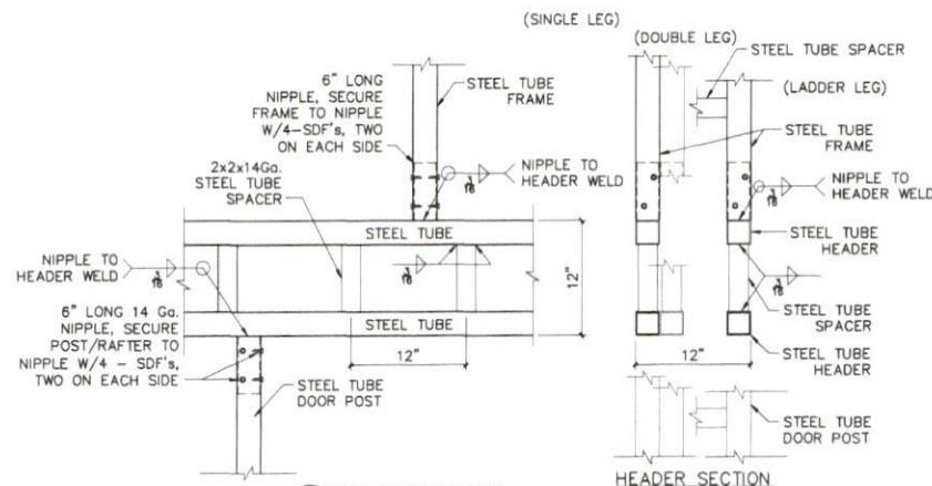
6 SIDE HEADER DETAIL
