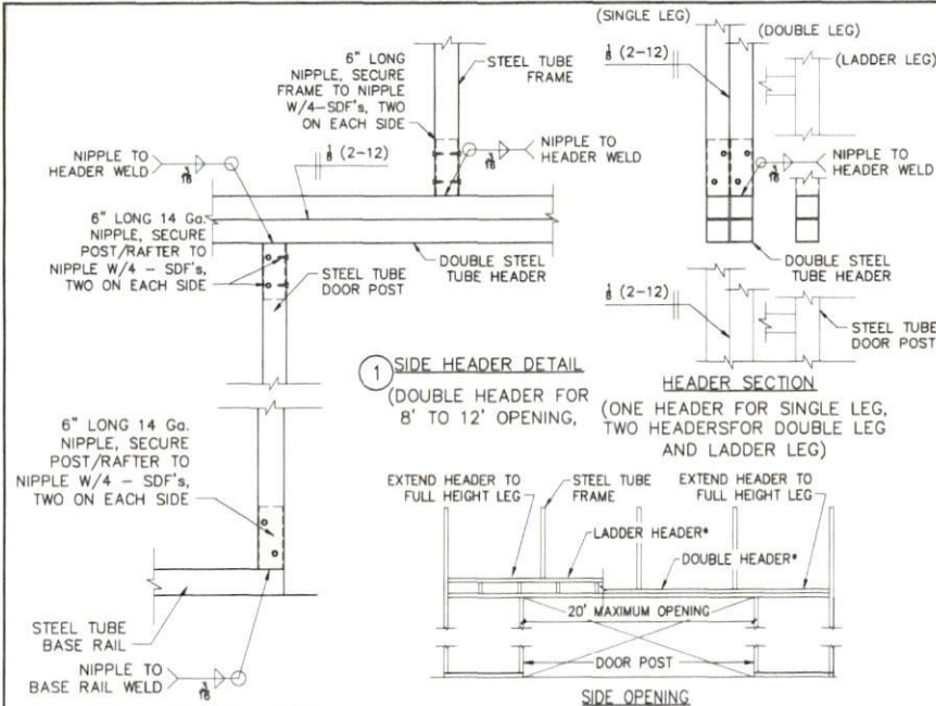
5 POST/BASE RAIL DETAIL
