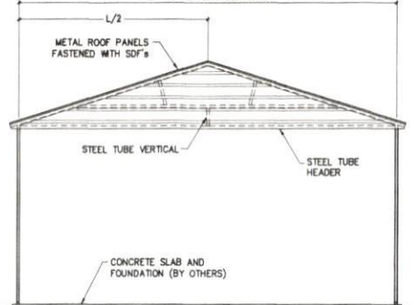
GABLE END ELEVATION
