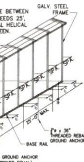
HELICAL GROUND ANCHORS
