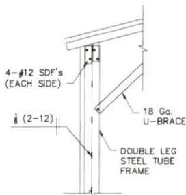
***DOUBLE LEG (LEG HEIGHTS 15' to 16')
