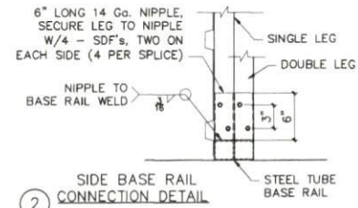
2 SIDE BASE RAIL CONNECTION DETAIL
