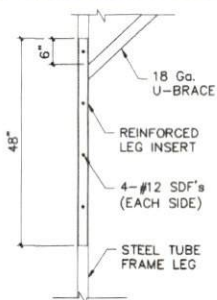
***REINFORCED LEG INSERT (LEG HEIGHTS 13' to 14')
