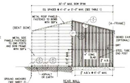
REAR WALL
