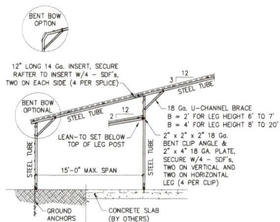
TYPICAL SIDE EXTENSION SECTION
