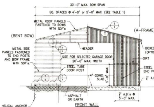
FRONT WALL
