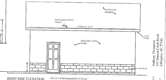
RIGHT SIDE ELEVATION Scale: 1/4" = 1'-0" All LVL's & Post-Engineered Roof Trusses To Be Designed By Supplier
