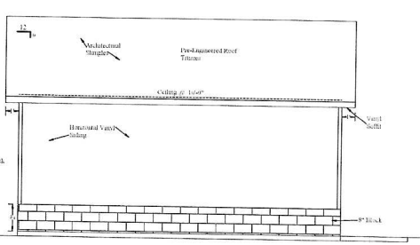
LEFT SIDE ELEVATION Scale: 1/4" = 1'-0" All LVL's & Post-Engineered Roof Trusses To Be Designed By Supplier
