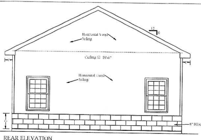
REAR ELEVATION Scale: 1/4" = 1'-0" All LVL's & Post-Engineered Roof Trusses To Be Designed By Supplier
