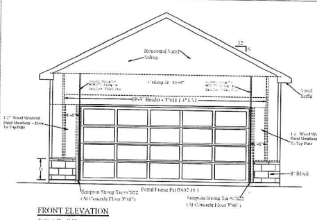
FRONT ELEVATION Scale: 1/4" = 1'-0" All LVL's & Post-Engineered Roof Trusses To Be Designed By Supplier
