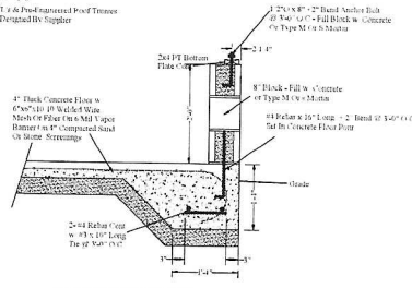
TYPICAL LVL FOOTING See Note
