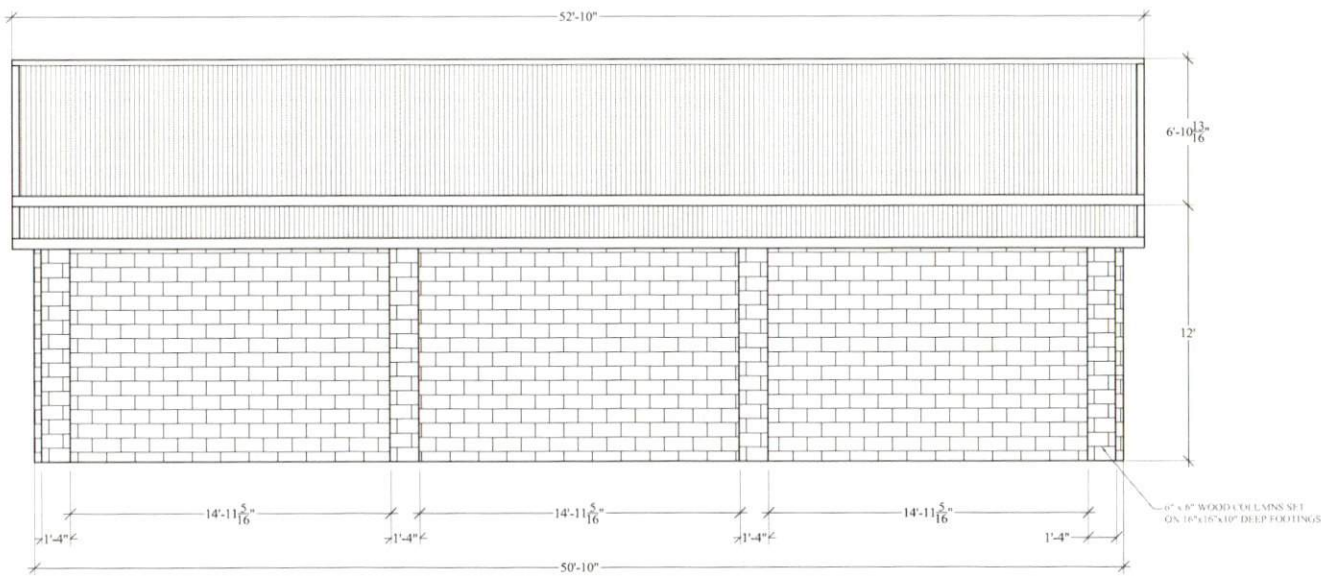
2 ELEVATION 3/16" = 1'-0"
