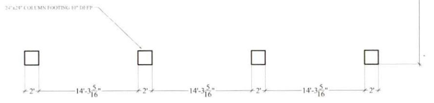
1 FOUNDATION PLAN 1/8" = 1'-0"
