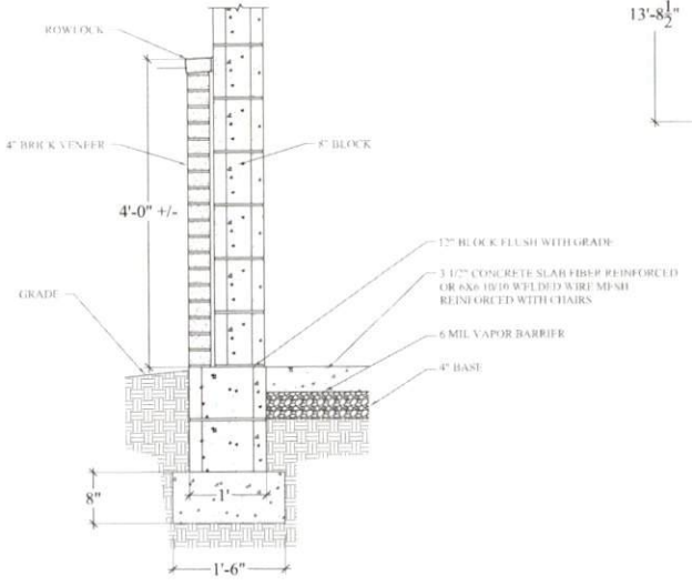
1 FOUNDATION SECTION 1/2" = 1'-0"
