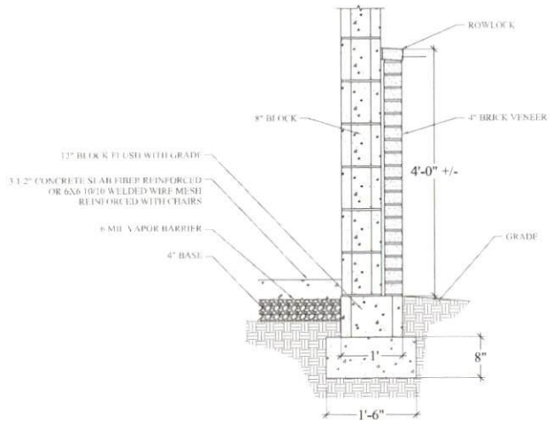
2 FOUNDATION SECTION 1/2" = 1'-0"
