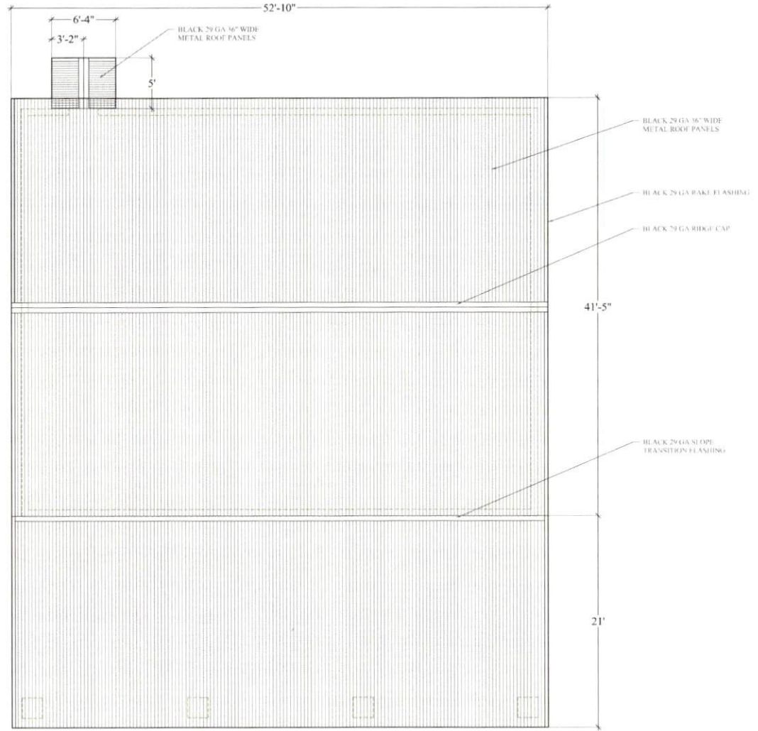
1 ROOF PLAN 1/8" = 1'-0"
