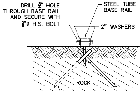
1 SOIL BASE RAIL ANCHOR DETAIL
