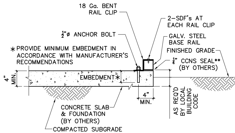
2C ALTERNATE BASE RAIL ANCHORAGE
