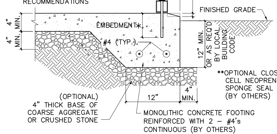
2 CONCRETE BASE RAIL ANCHORAGE (SINGLE LEG)
