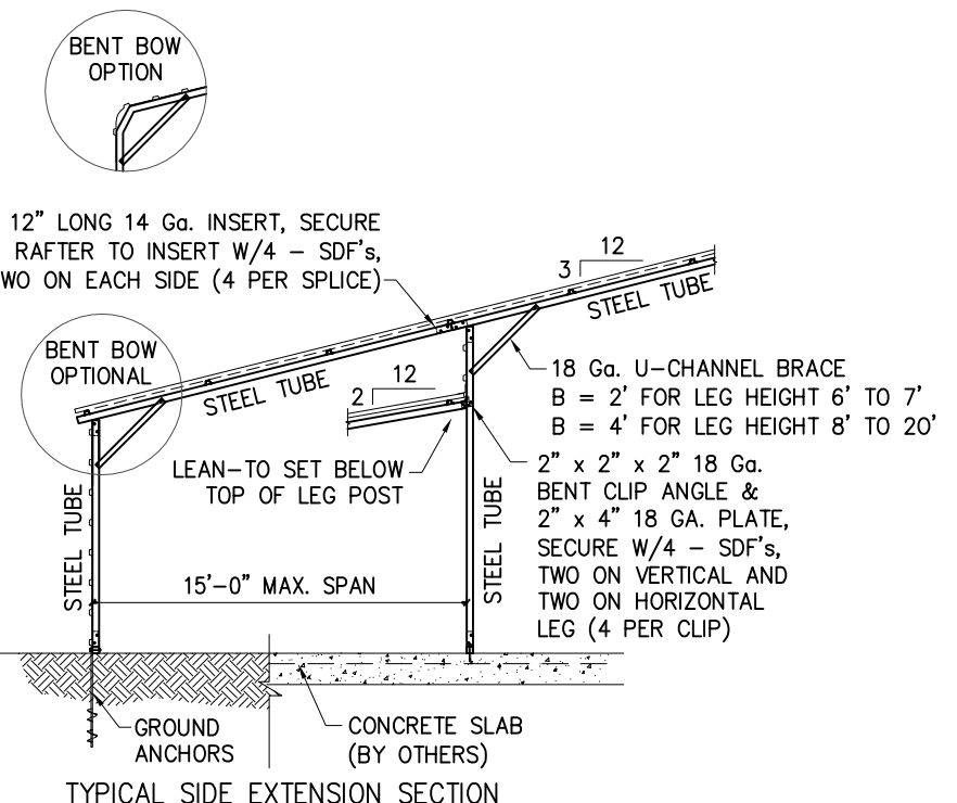
TYPICAL SIDE EXTENSION SECTION
