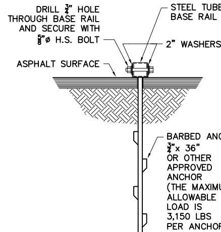
1 SOIL BASE RAIL ANCHOR DETAIL
