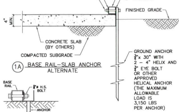
ALTERNATE DETAIL
