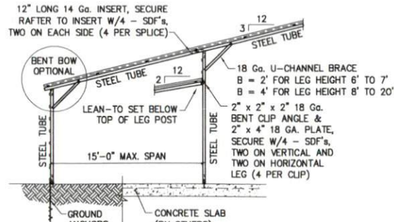
TYPICAL SIDE EXTENSION SECTION
