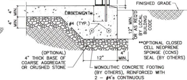
2B CONCRETE BASE RAIL ANCHORAGE (DOUBLE LEG)
