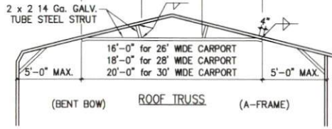
1 2 TYPICAL BOW SECTION
