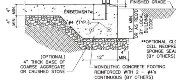
2 CONCRETE BASE RAIL ANCHORAGE (SINGLE LEG)
