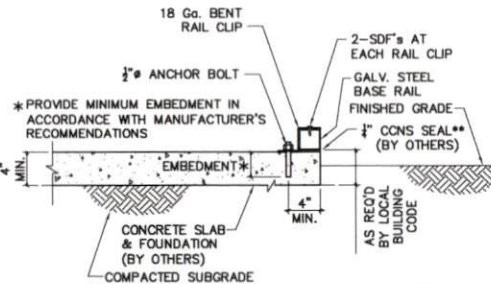
2C ALTERNATE BASE RAIL ANCHORAGE
