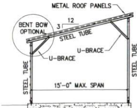
STAND-ALONE LEAN-TO
