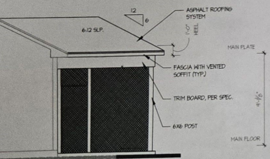
PPO - LEFT SIDE ELEVATION SCREENED PORCH (RALEIGH)
