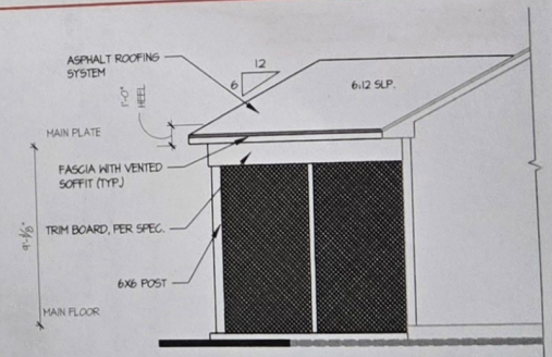
PPO - RIGHT SIDE ELEVATION SCREENED PORCH (RALEIGH)
