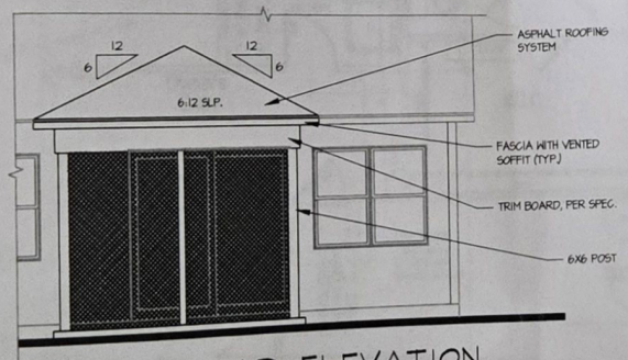
PPO - REAR ELEVATION SCREENED PORCH (RALEIGH)
