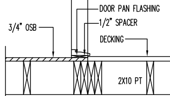
DOOR INSTALLATION @ FACT BUILT PORCH
