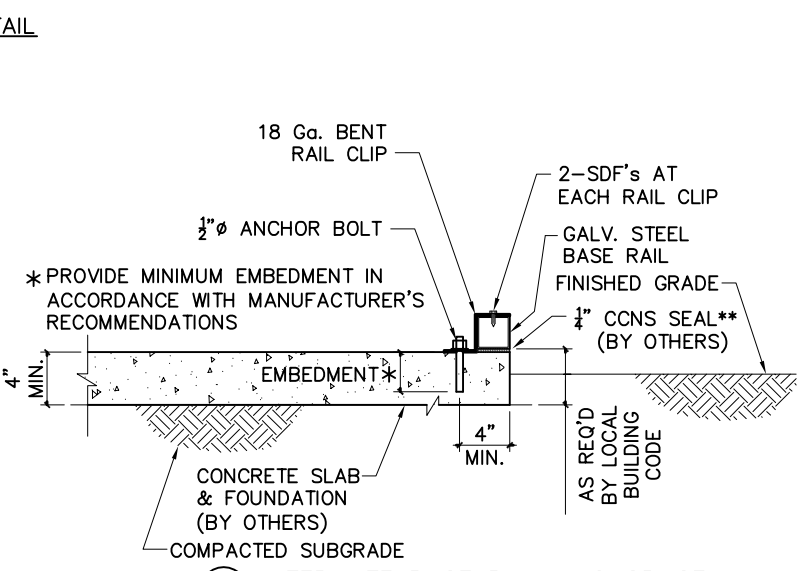
2C ALTERNATE BASE RAIL ANCHORAGE
