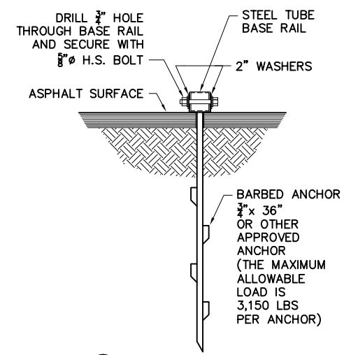
1B ASPHALT ANCHOR DETAIL
