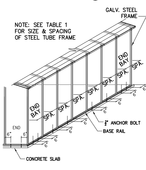
ANCHOR BOLTS
