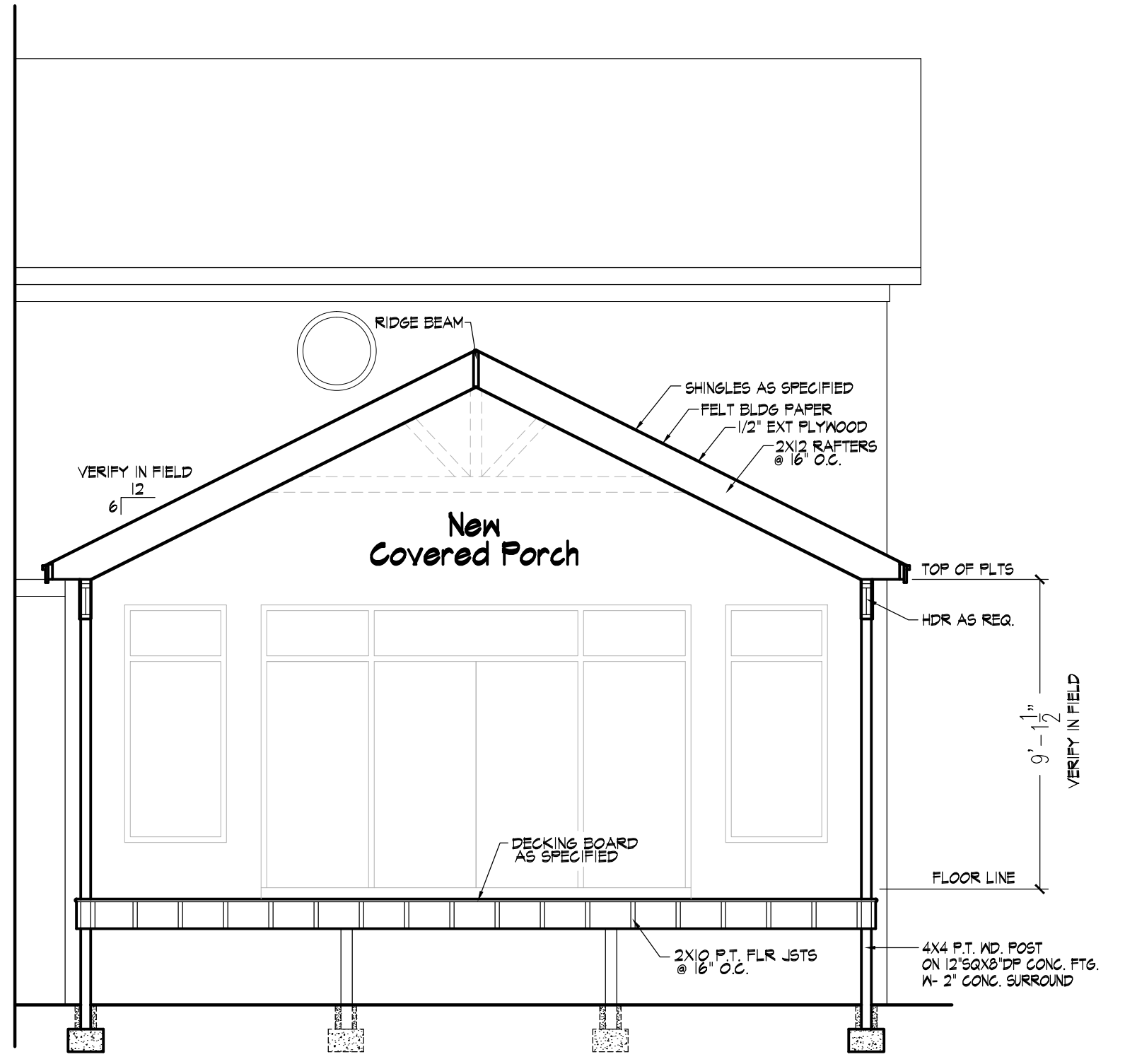
402 Building Section Scale: 1/4" = 1'-0"
