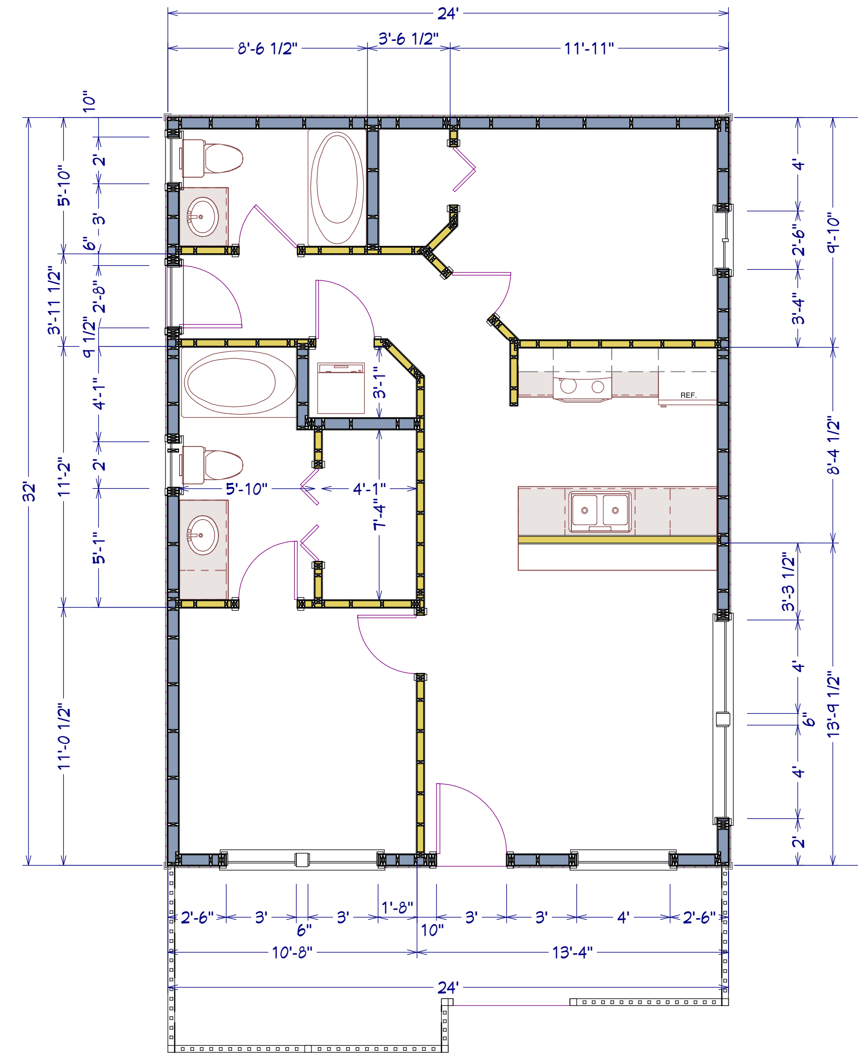
MAIN FLOOR PLAN SCALE: 1/4" = 1'
