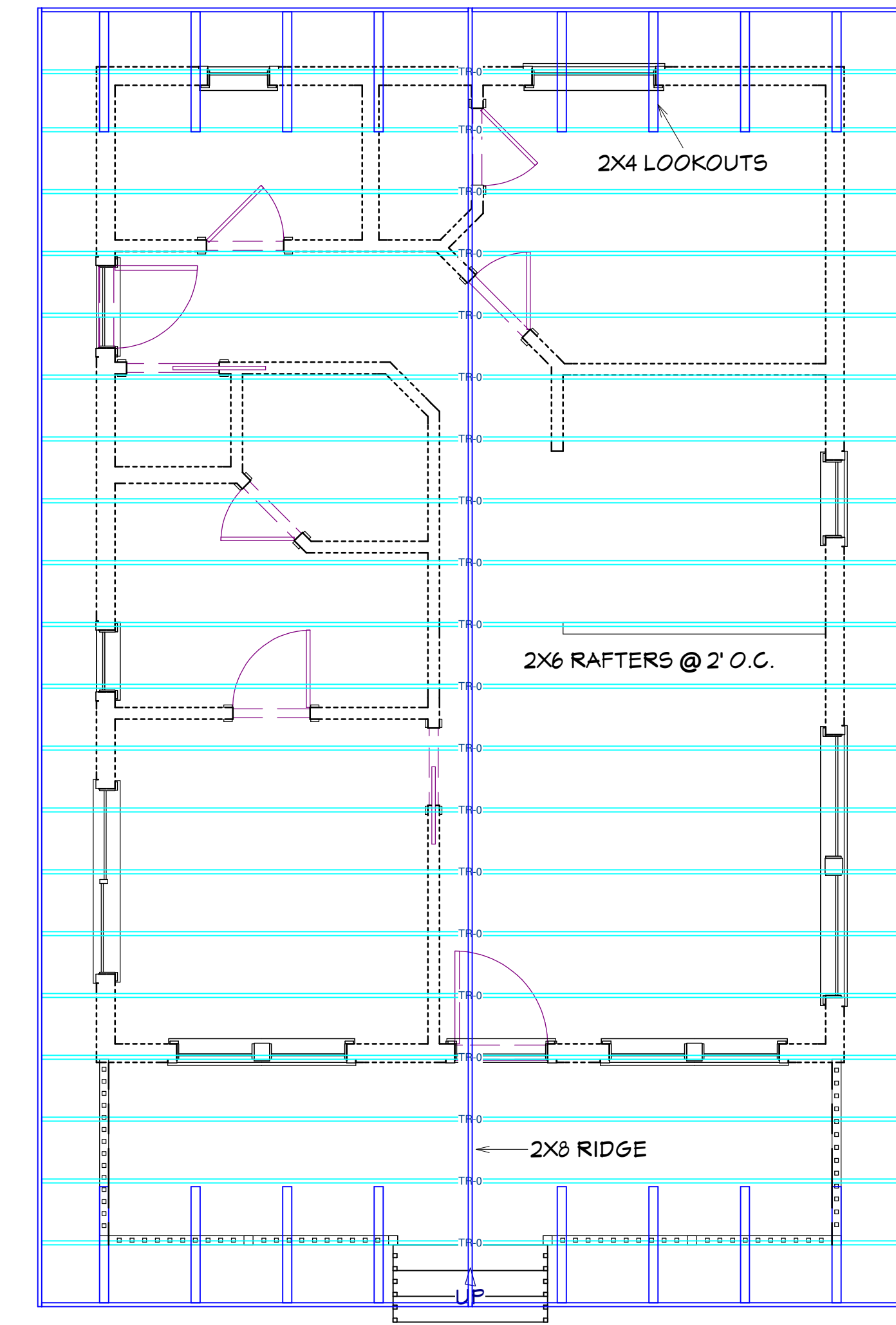
ROOF FRAMING PLAN SCALE: 1/4" = 1'
