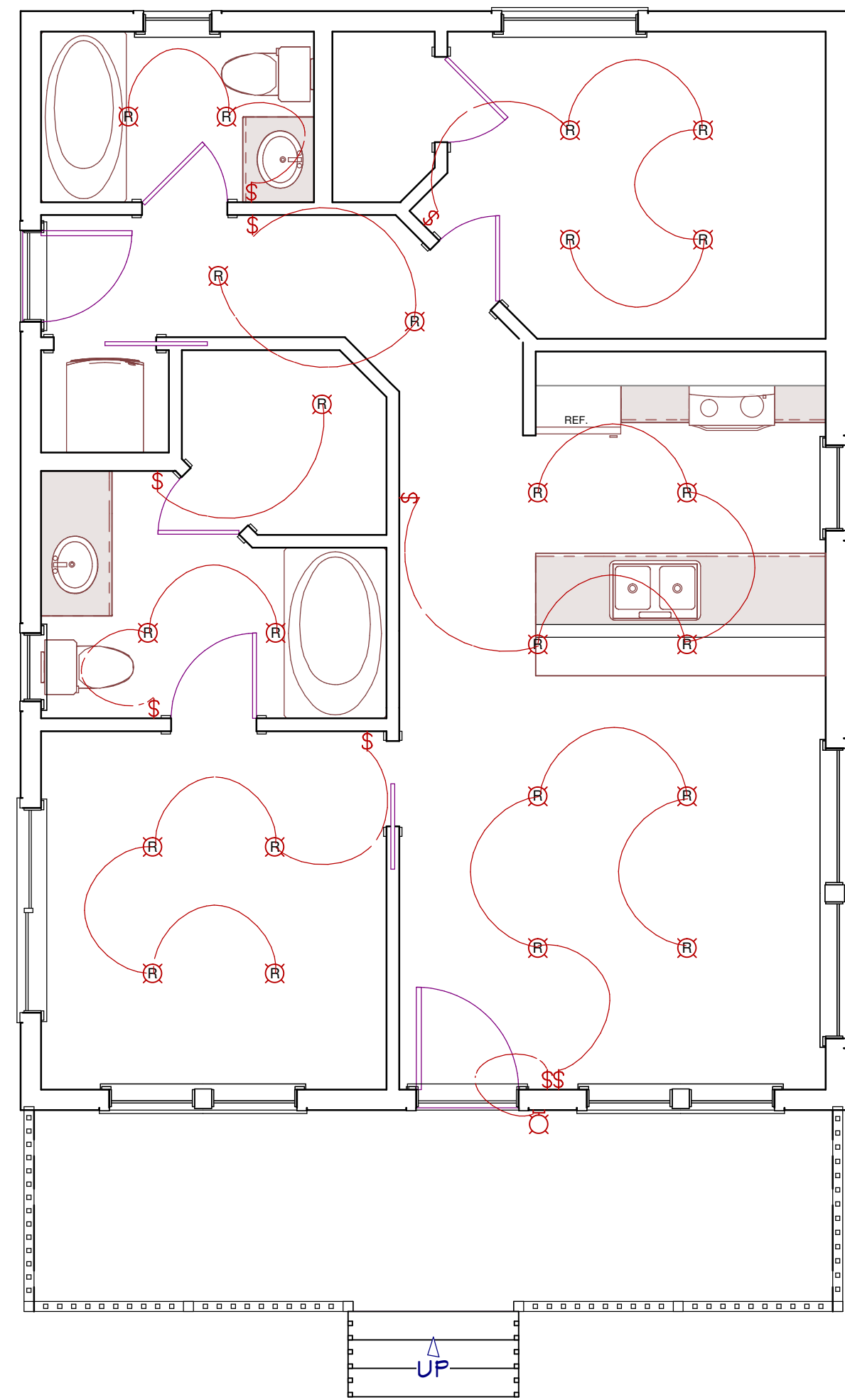
LIGHTING PLAN SCALE: 1/4" = 1'
