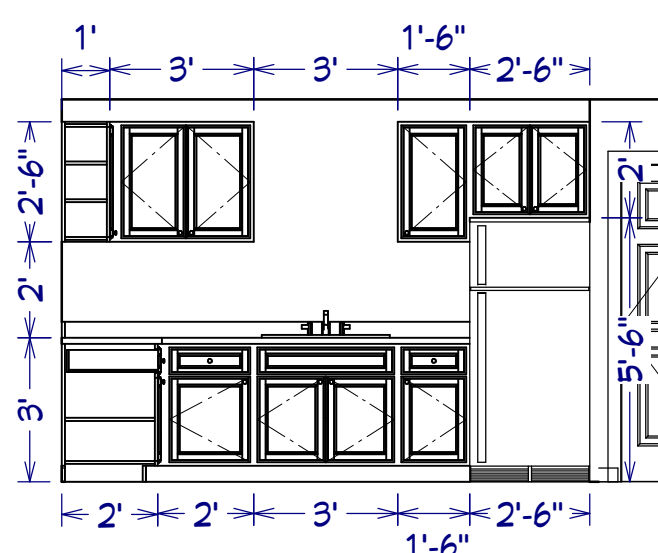
CABINET ELEVATION B SCALE: 1/4" = 1'
