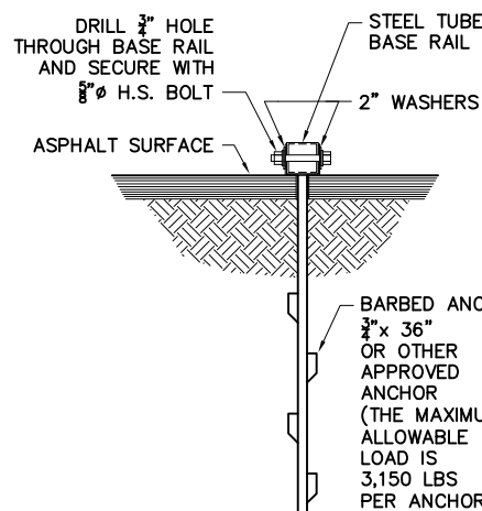
1B ASPHALT ANCHOR DETAIL
