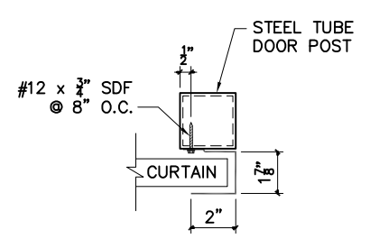
SECTION THROUGH ROLL-UP DOOR POST
