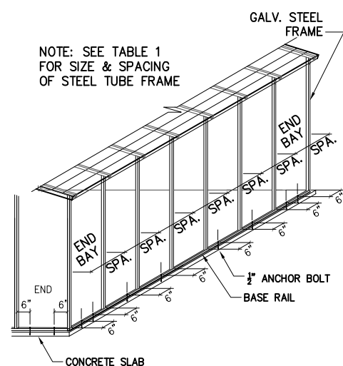
ANCHOR BOLTS
