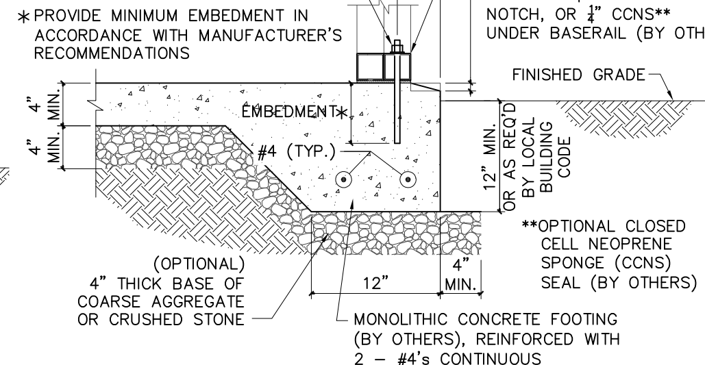
2B CONCRETE BASE RAIL ANCHORAGE (DOUBLE LEG)
