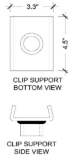
Figure 5 - Clip Support
