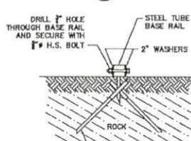
1 SOIL BASE RAIL ANCHOR DETAIL
