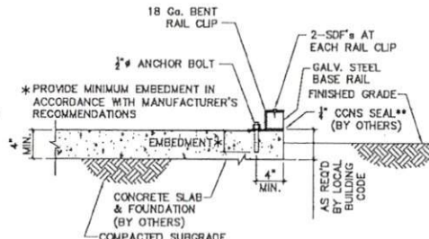
2C ALTERNATE BASE RAIL ANCHORAGE
