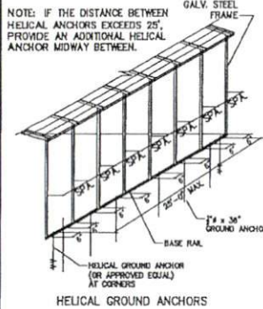
HELICAL GROUND ANCHORS
