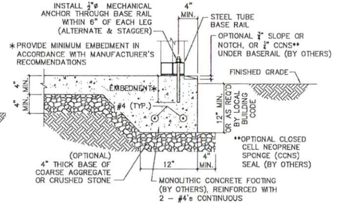
2B CONCRETE BASE RAIL ANCHORAGE (DOUBLE LEG)
