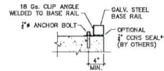
2D ALTERNATE BASE RAIL CLIP
