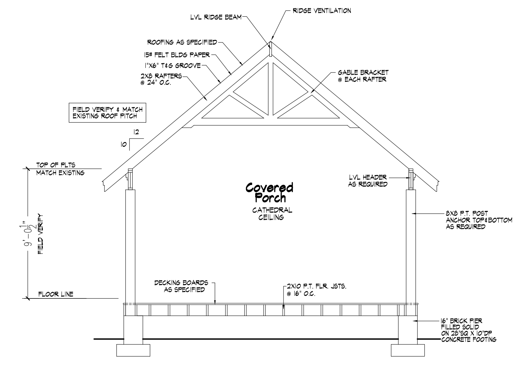
603 Building Section Scale: 1/4" = 1'-0"
