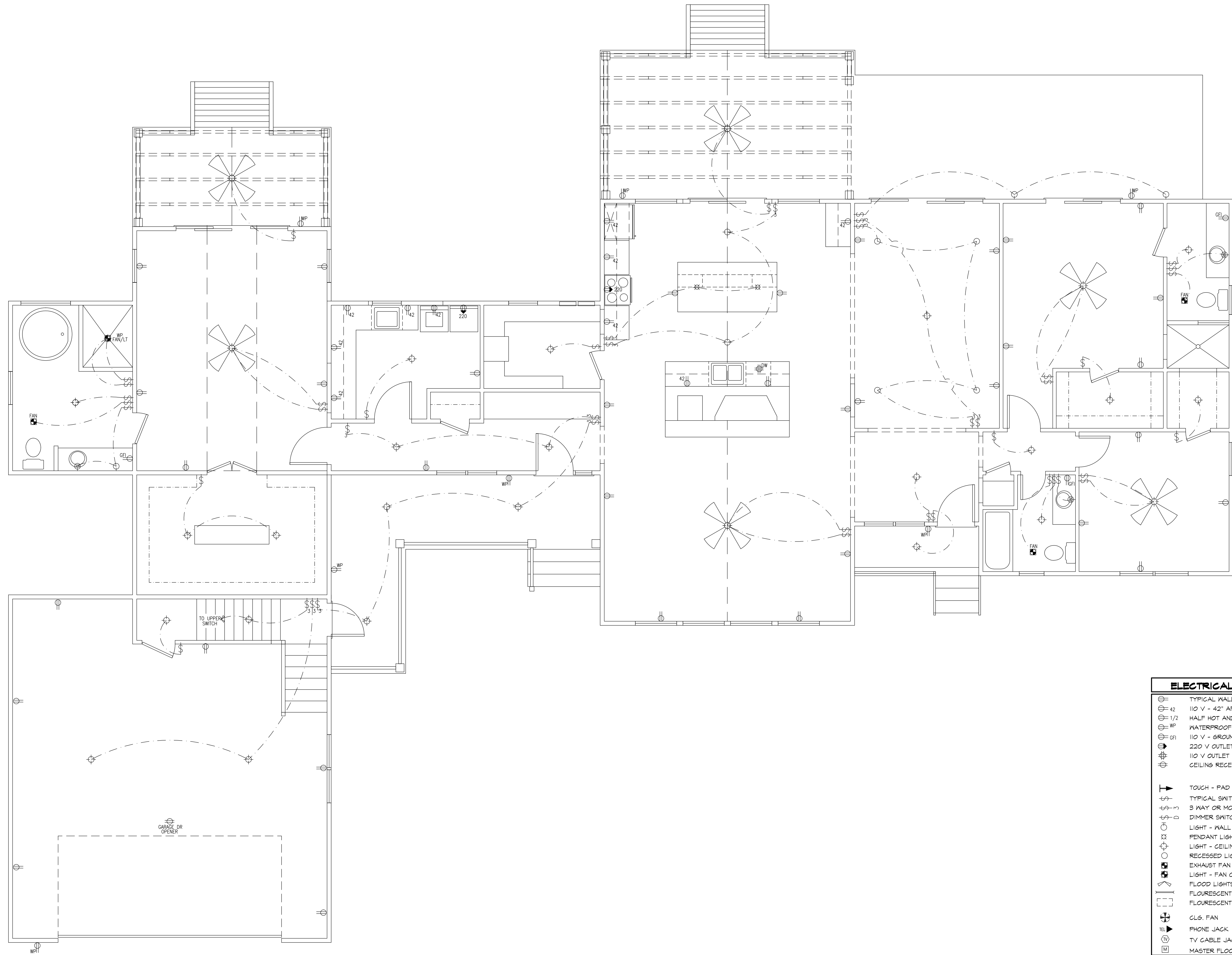
101 Electrical Floor Plan Scale: 1/4" = 1'-0"
