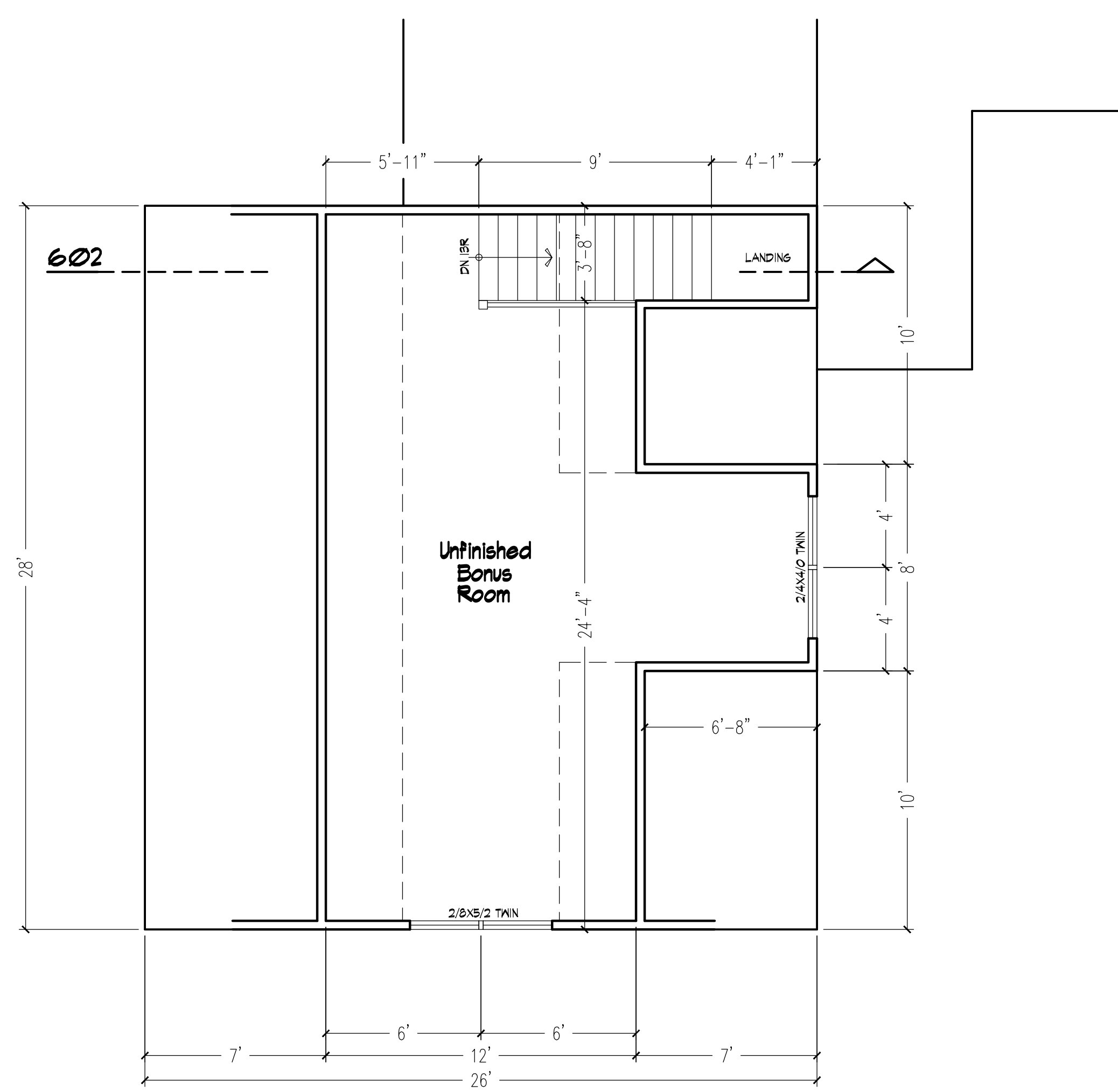
601 Bonus Room Floor Plan Scale: 1/4" = 1'-0"
