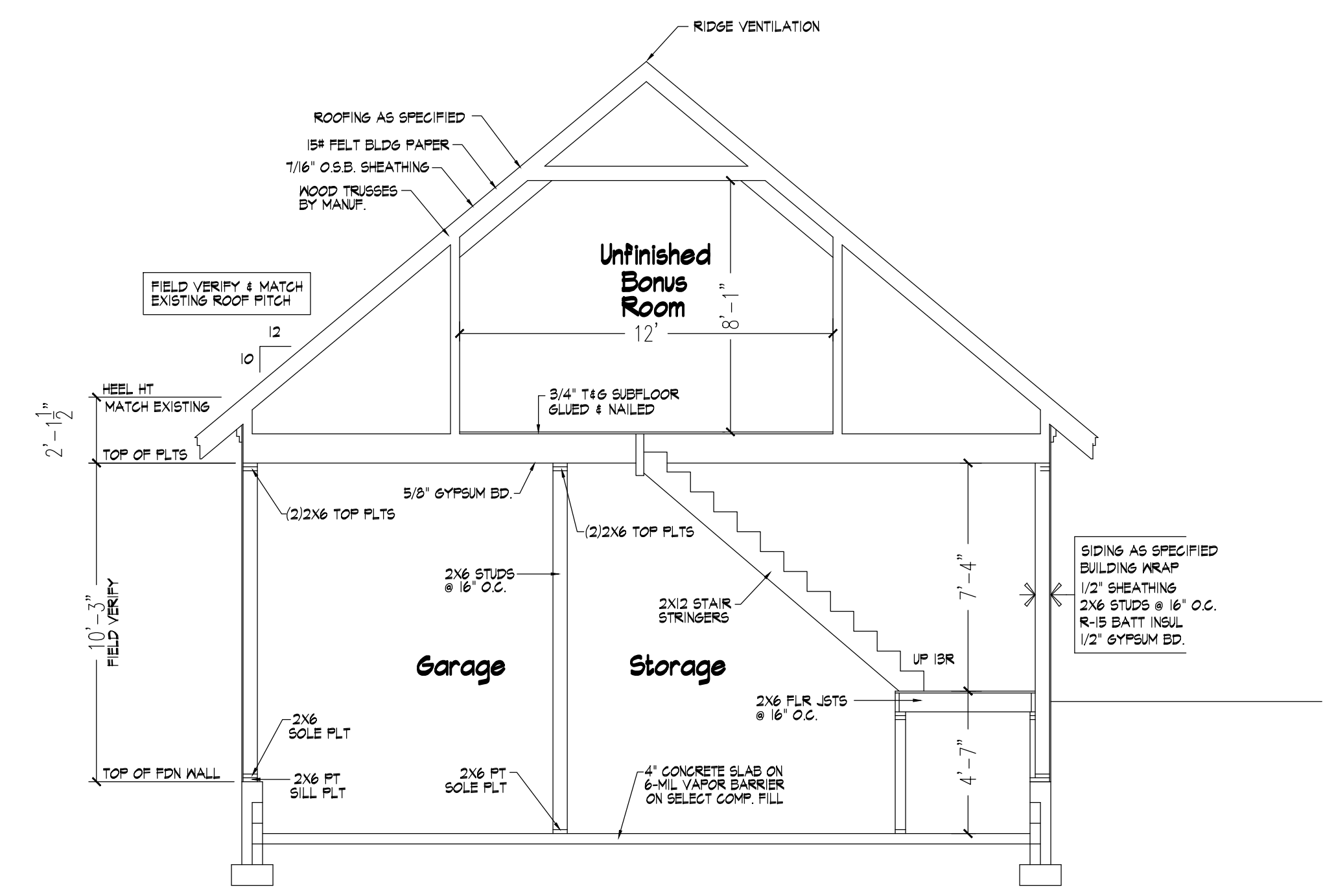
604 Building Section Scale: 1/4" = 1'-0"
