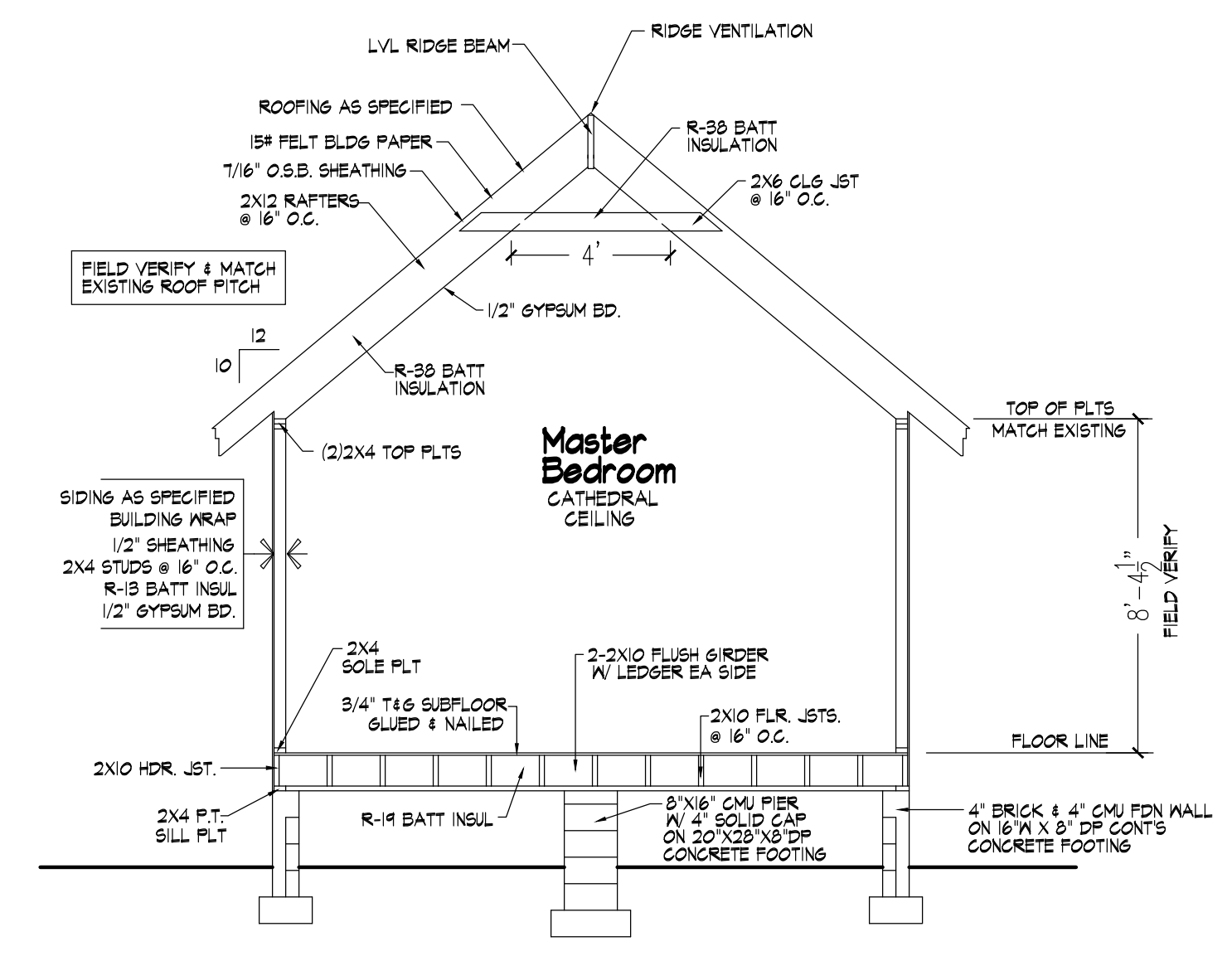
602 Building Section Scale: 1/4" = 1'-0"
