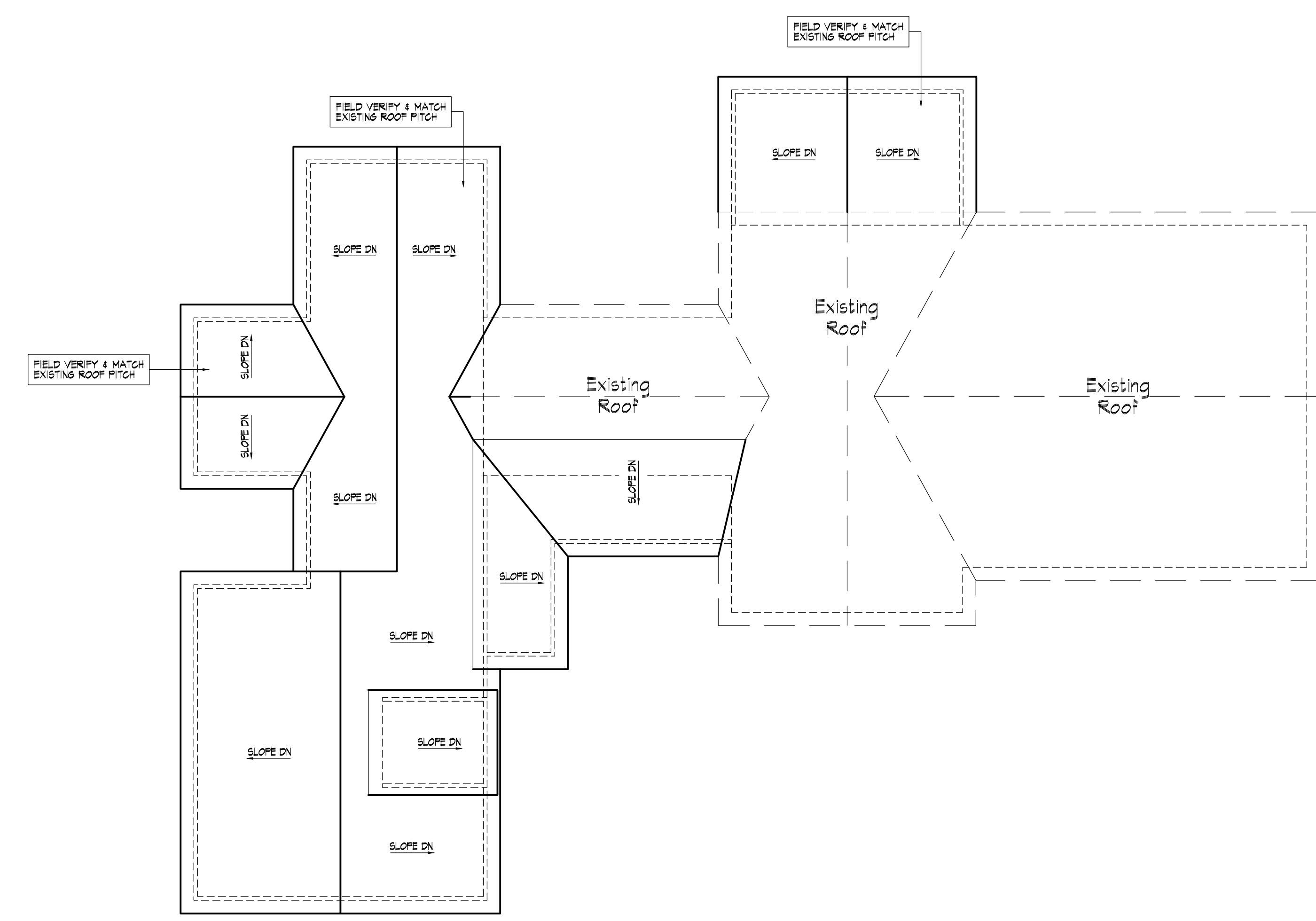
605 Roof Plan Scale: 1/8" = 1'-0"
