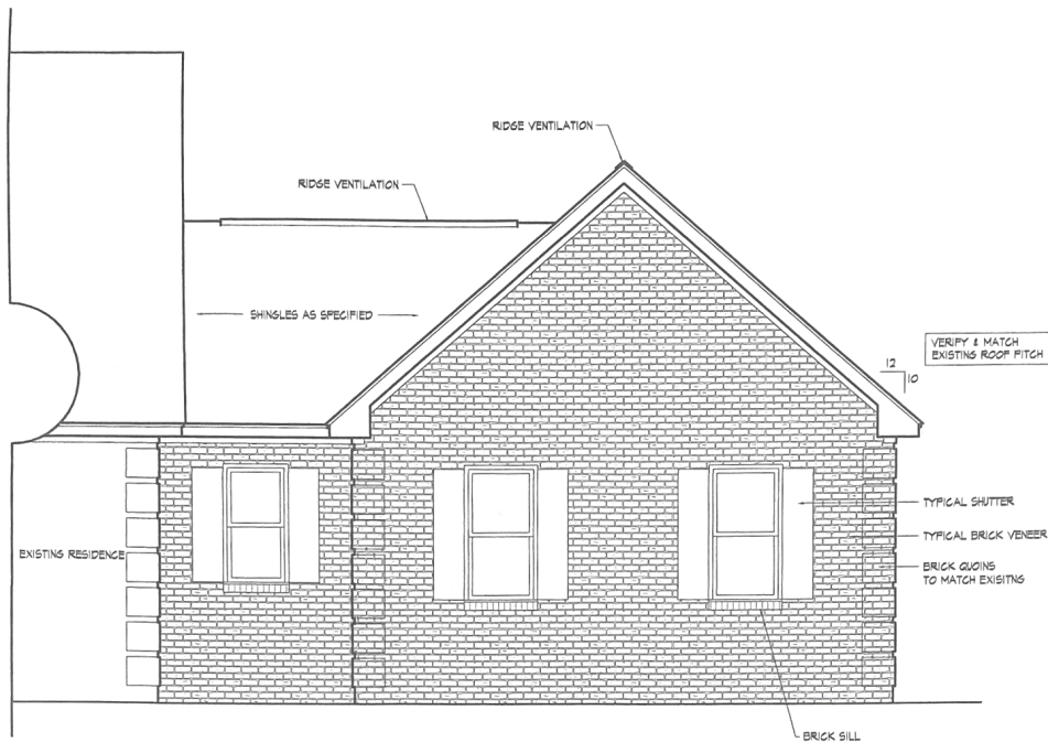
101 Front Elevation
