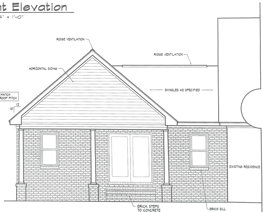
103 Rear Elevation
