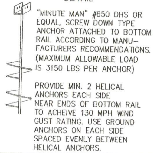
HELICAL ANCHOR DETAIL
