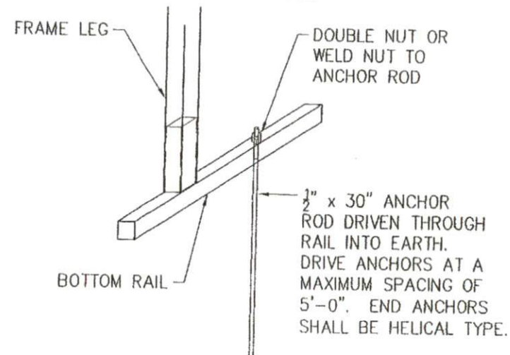
GROUND ANCHOR DETAIL
