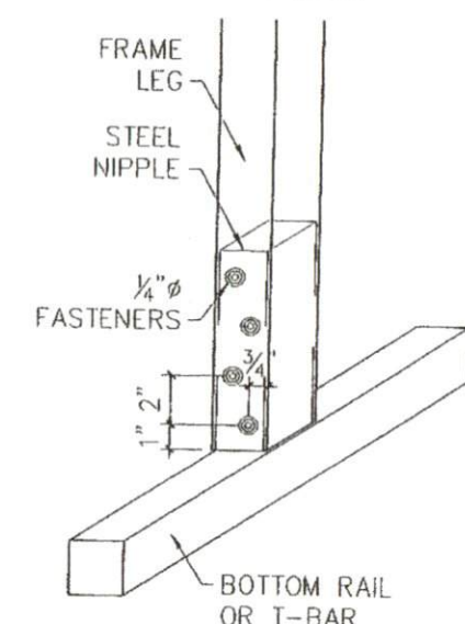
FRAME CONNECTION
