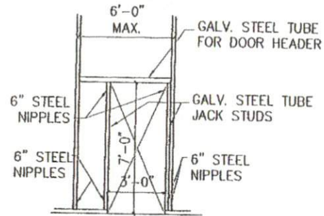
STANDARD DOOR OPENING
