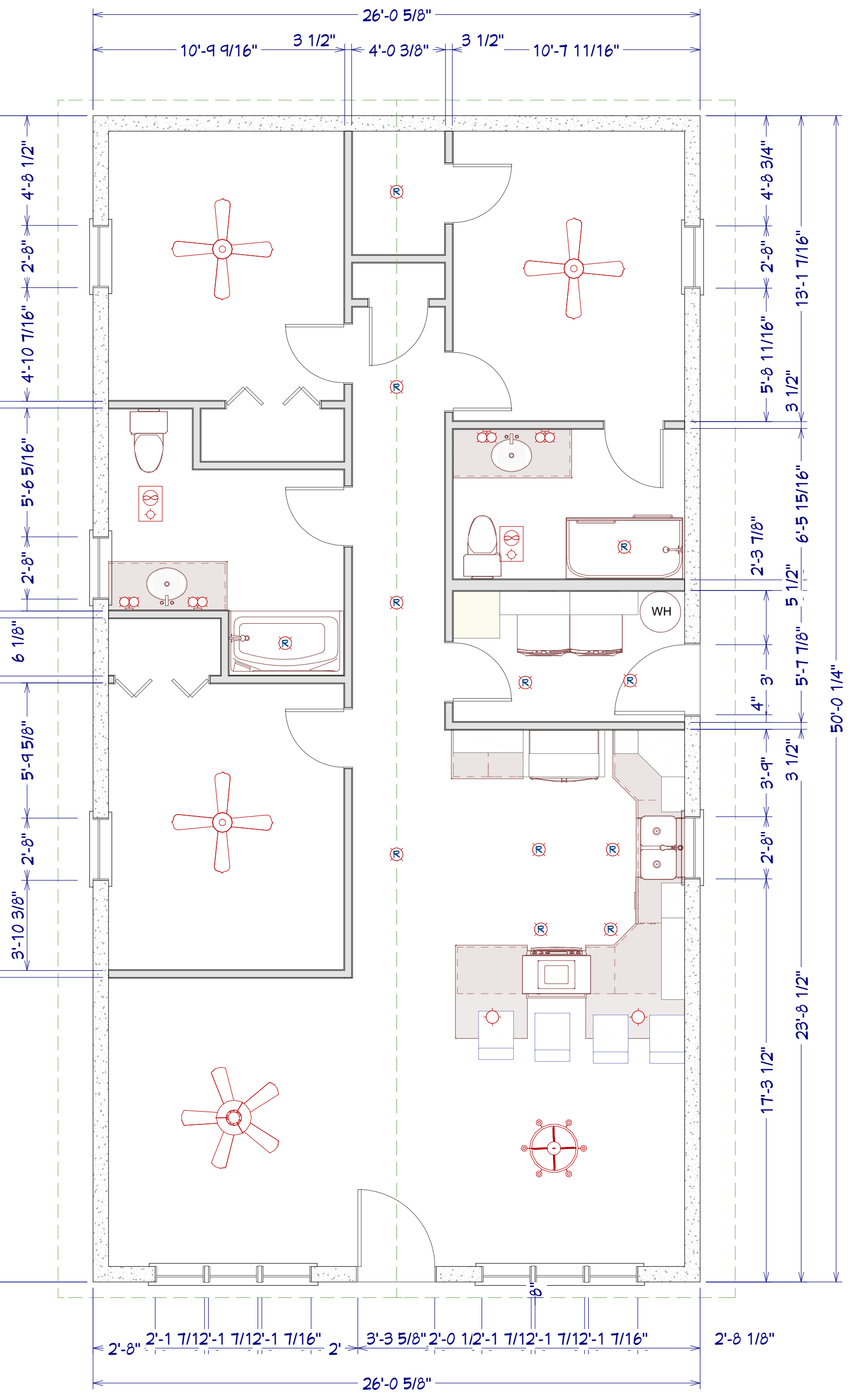
LIVING AREA 1303 SQ FT
