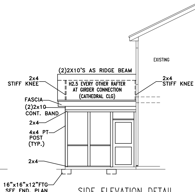
SIDE ELEVATION DETAIL SCALE:.....1/4"=1'
