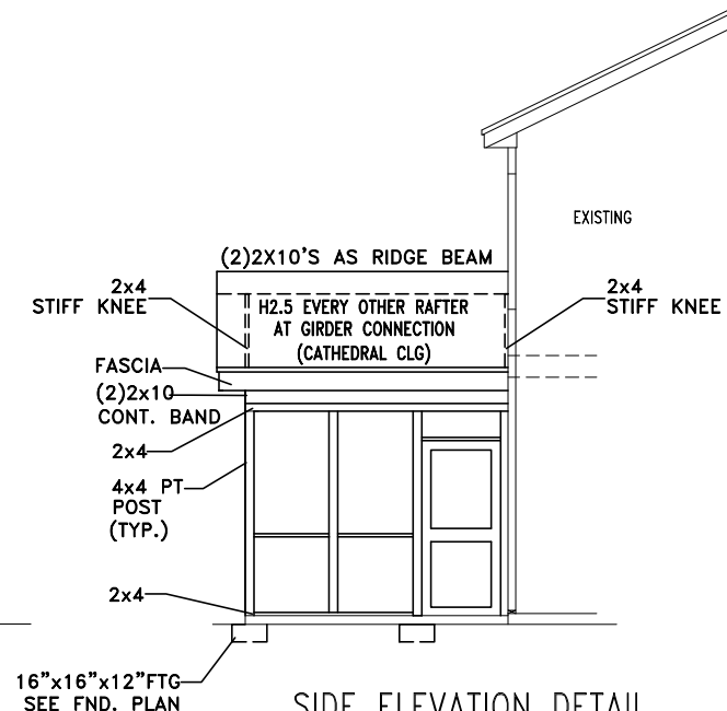
SIDE ELEVATION DETAIL SCALE:.....1/4"=1'
