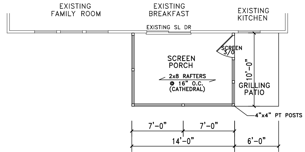
FLOOR PLAN DETAIL SCALE:.....1/4"=1'
