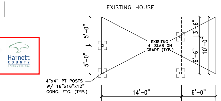
FOUNDATION SCALE:.....1/4"=1'
