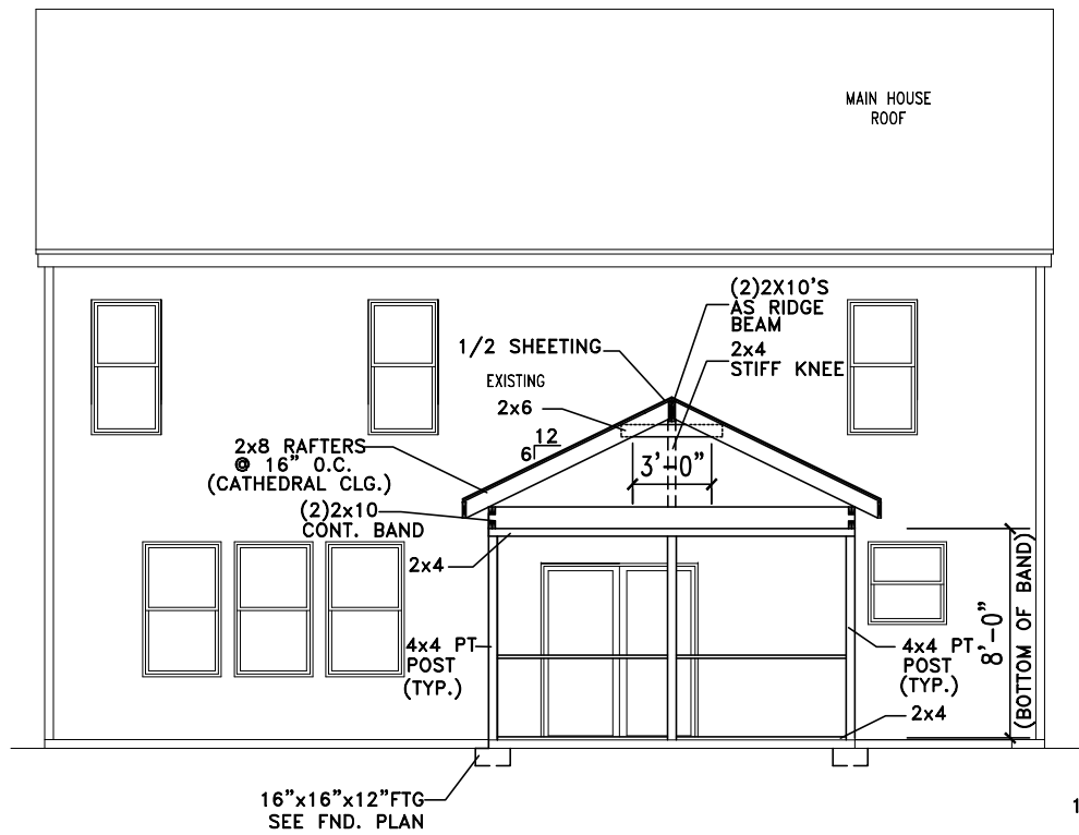
FRONT ELEVATION DETAIL SCALE:.....1/4"=1'
