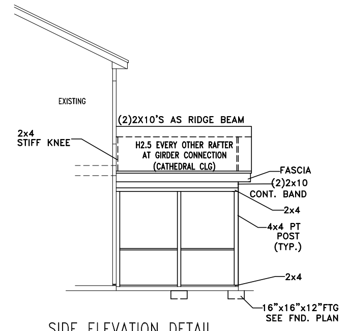
SIDE ELEVATION DETAIL SCALE:.....1/4"=1'
