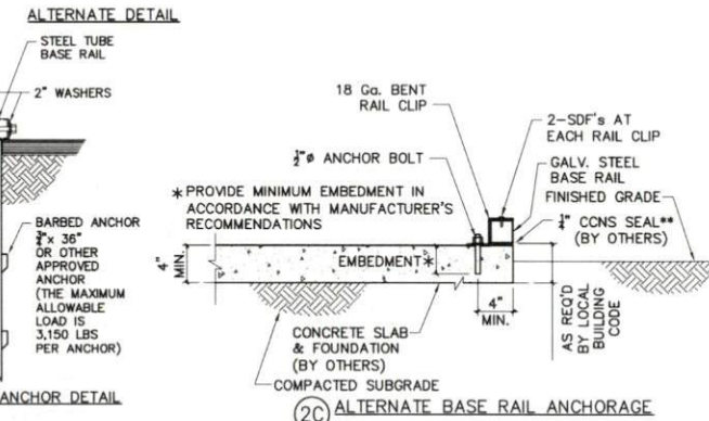
2C ALTERNATE BASE RAIL ANCHORAGE
