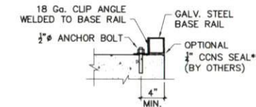
2D ALTERNATE BASE RAIL CLIP
