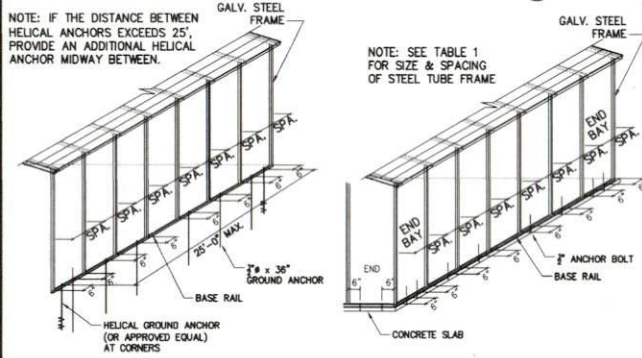
HELICAL GROUND ANCHORS
