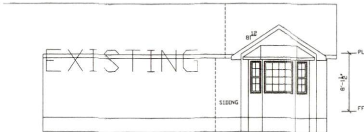
FRONT ELEVATION SCALE: 1/4"=1'
