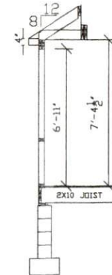
BAY WINDOW SECTION SCALE: 1/2"=1'
