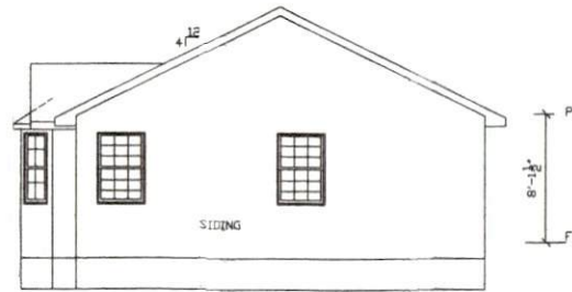
RIGHT SIDE ELEVATION SCALE: 1/4"=1'
