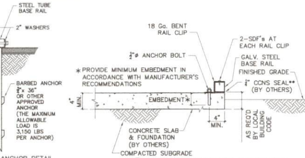
1B ASPHALT ANCHOR DETAIL
