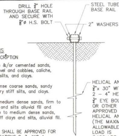
1 SOIL BASE RAIL ANCHOR DETAIL
