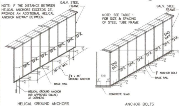
HELICAL GROUND ANCHORS
