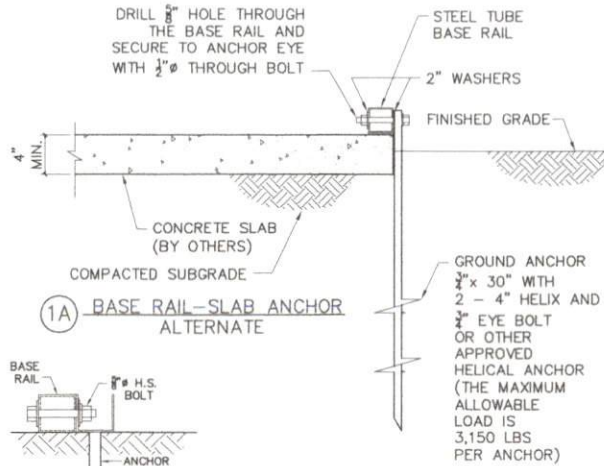
1A BASE RAIL-SLAB ANCHOR ALTERNATE
