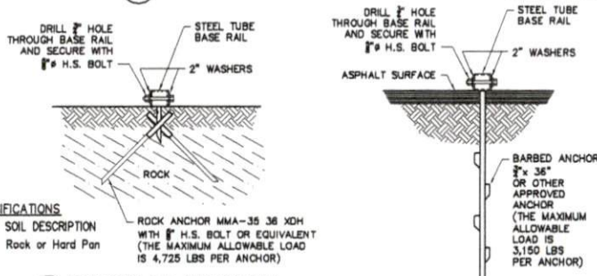
1C ROCK ANCHOR DETAIL
