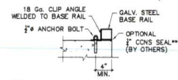
2D ALTERNATE BASE RAIL CLIP
