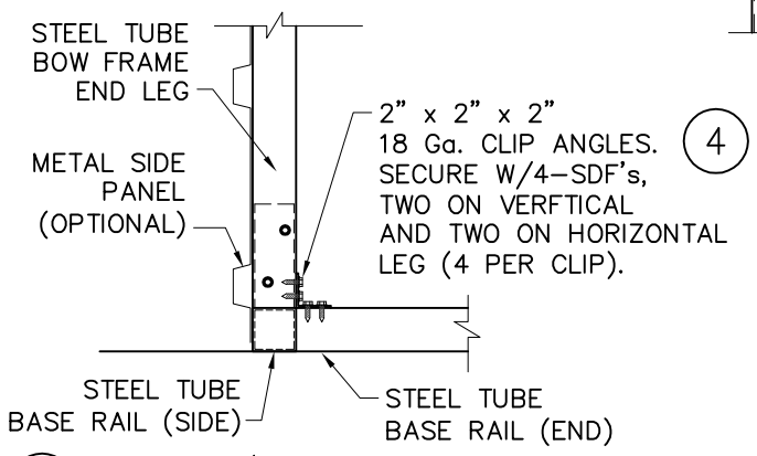
7 END BOW/BASE RAIL CONNECTION
