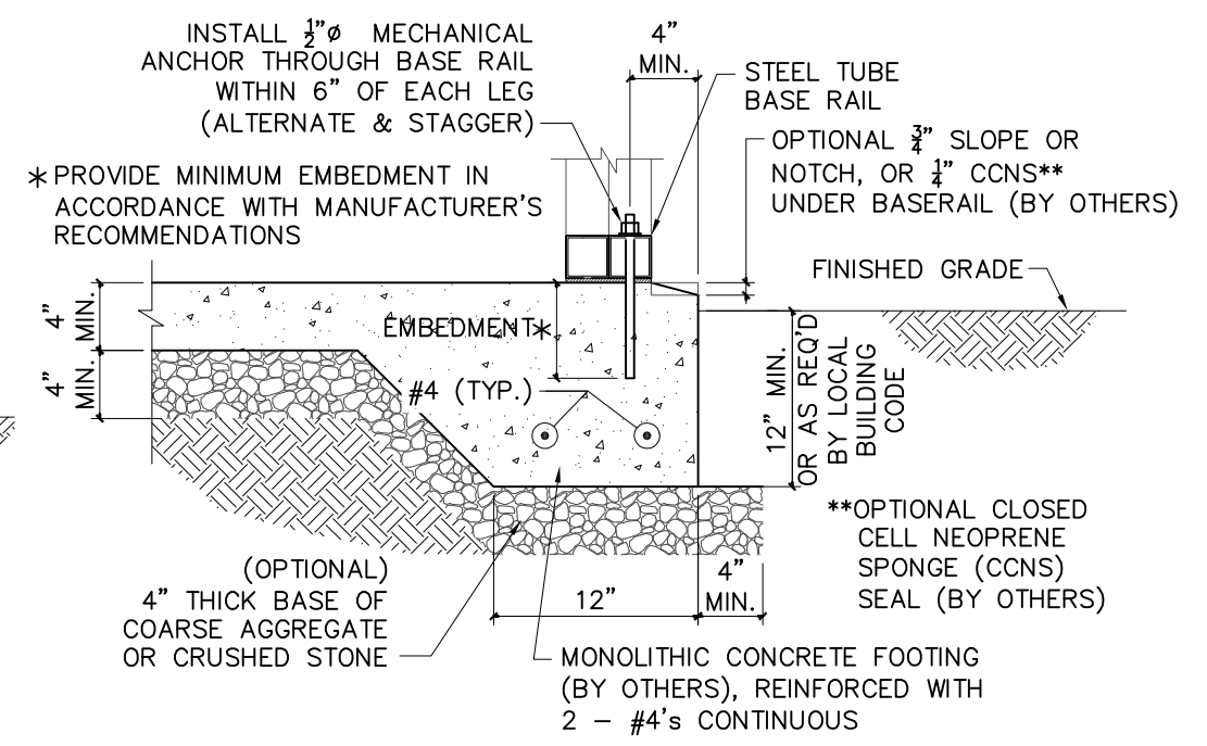
2B CONCRETE BASE RAIL ANCHORAGE (DOUBLE LEG)
