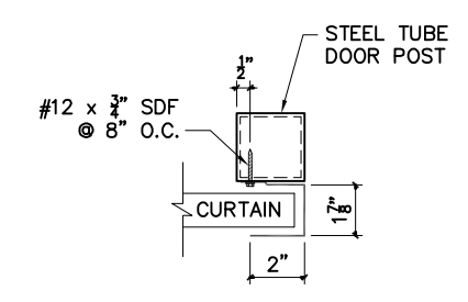
SECTION THROUGH ROLL-UP DOOR POST
