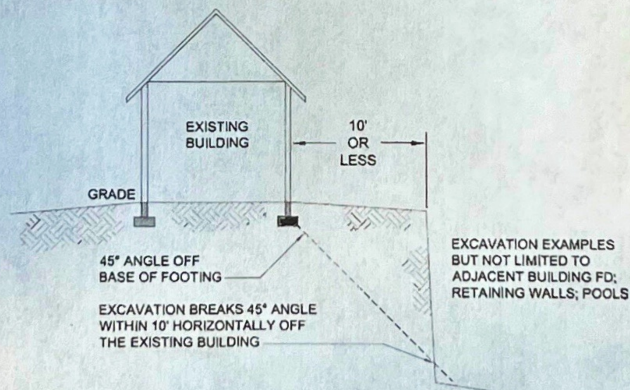
FIGURE R403.1.9 EXCAVATIONS NEAR FOOTINGS OR FOUNDATIONS
