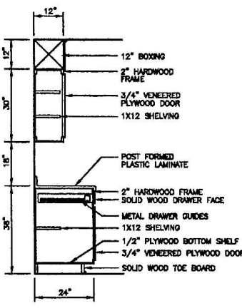
SECTION THRU KITCHEN CABINETS
