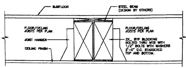
D004 SECTION THRU STEEL BEAM
