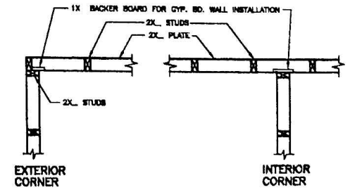
D008 DETAIL ADVANCED WALL FRAMING
