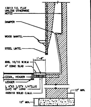
D006 SECT. THRU FIREPLACE ON WOOD FLOOR
