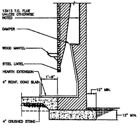
D005 SECT. THRU FIREPLACE ON CONCRETE SLAB
