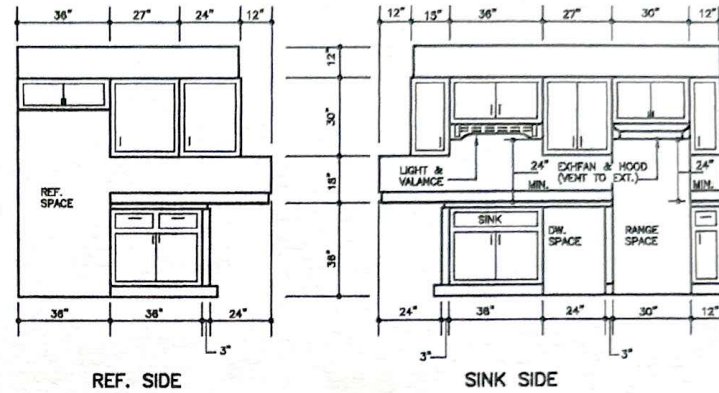
REF. SIDE KITCHEN CABINET ELEVATIONS SCALE 3/8" = 1'-0"
