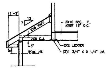
803 SECTION THRU FRONT SHED ROOF SCALE 3/8" = 1'-0"
