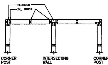
D007 DETAIL BASIC WALL FRAMING
