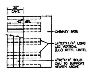
PLAN VIEW OF SUSPENDED HEARTH
