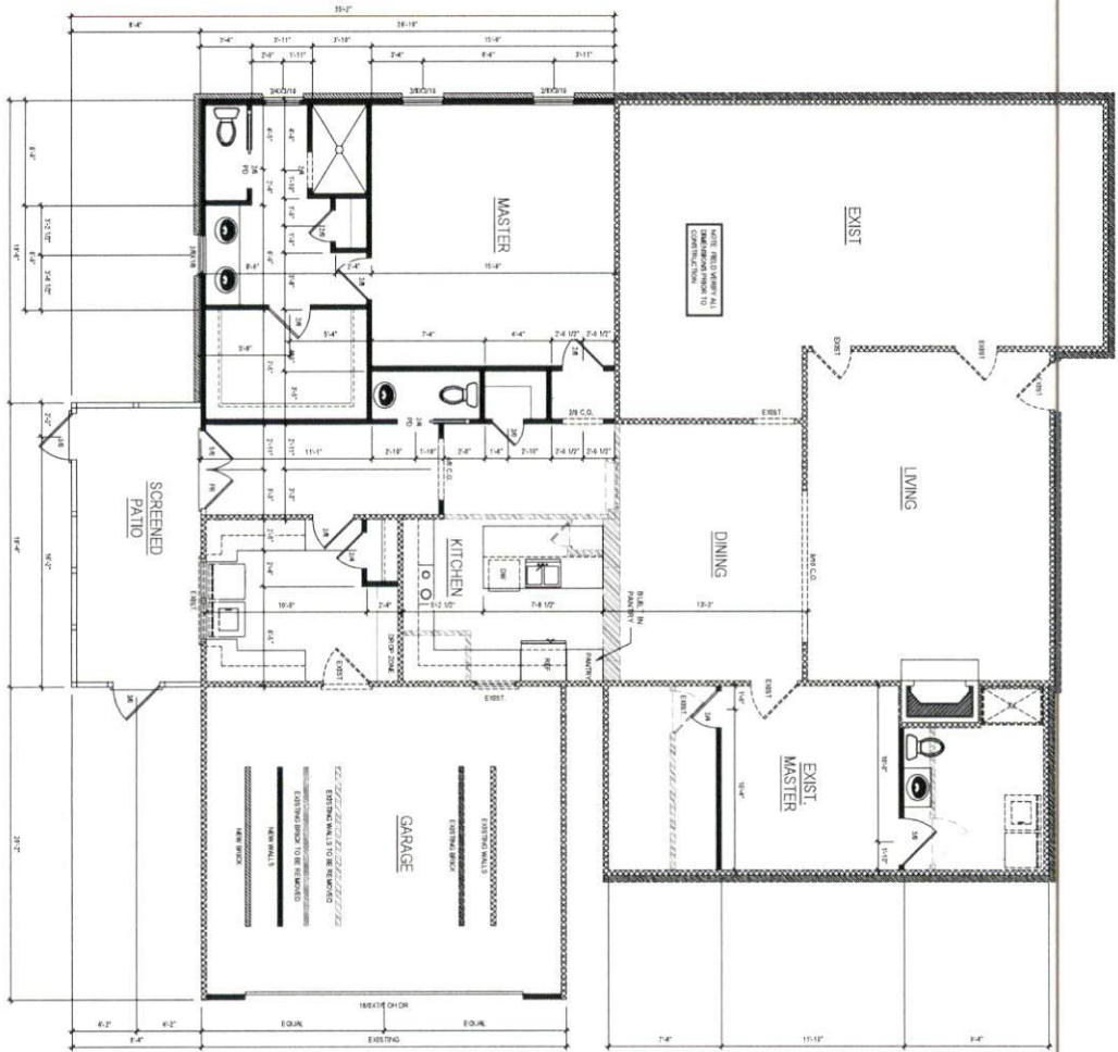
FIRST FLOOR PLAN 1/4" = 1'-0" CEILING HGT. = 8'-0"
