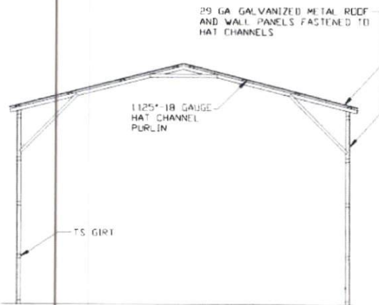
TYPICAL SECTION VERTICAL ROOF/SIDING OPTION
