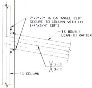
16 LEAN-TO RAFTER TO RAFTER POST CONNECTION DETAIL FOR WIDTHS 12'-0" < TO ≤ 16'-0" SCALE: NTS
