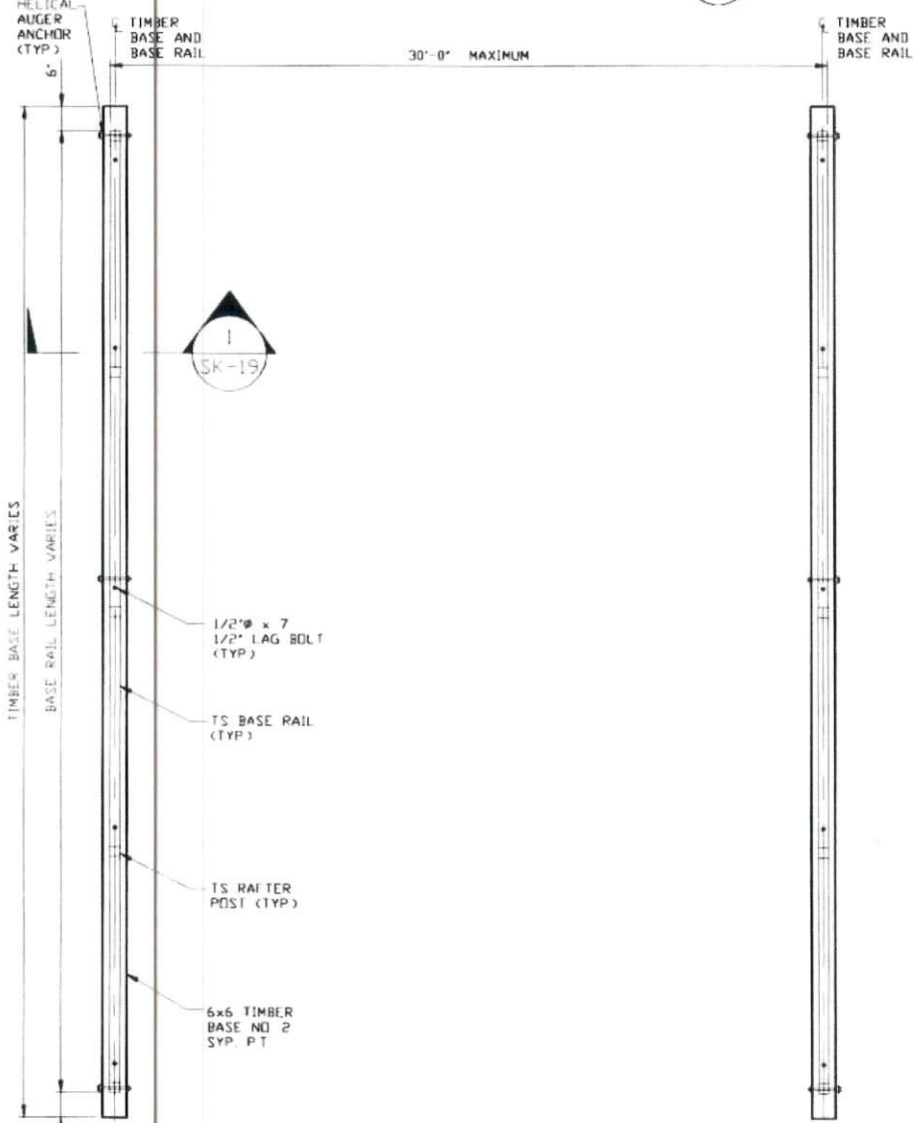
TIMBER FOOTING PLAN SCALE: NTS
