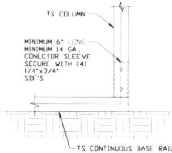
COLUMN/BASE RAIL CONNECTION DETAIL
