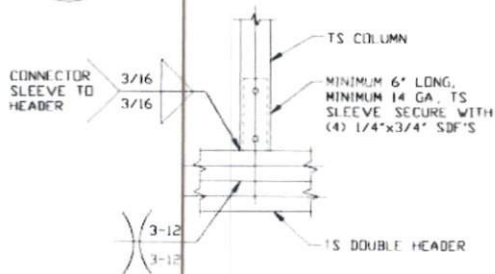
COLUMN/DOUBLE HEADER CONNECTION DETAIL
