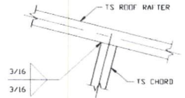
RAFTER TO CHORD CONNECTION DETAIL
