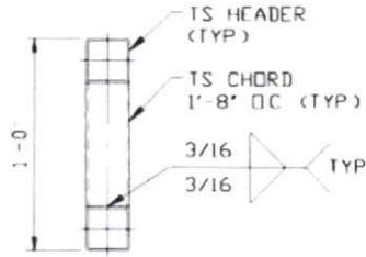
LACED HEADER DETAIL FOR DOOR OPENINGS 12'-0" < LENGTH ≤ 20'-0"
