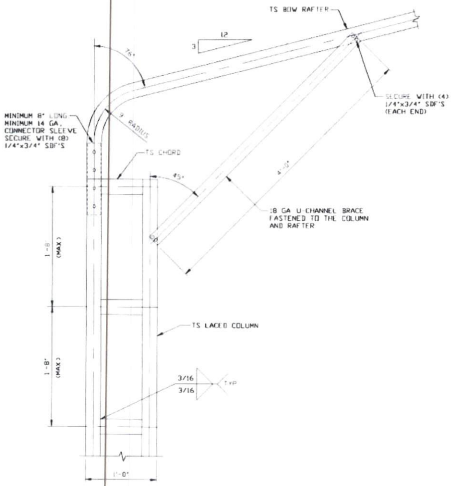
BOX EAVE RAFTER/CORNER POST CONNECTION DETAIL FOR HEIGHTS 16'-0" < TO ≤ 20'-0" SCALE: NTS
