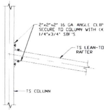
16A LEAN-TO RAFTER TO RAFTER POST CONNECTION DETAIL FOR WIDTHS ≤ 12'-0" SCALE: NTS
