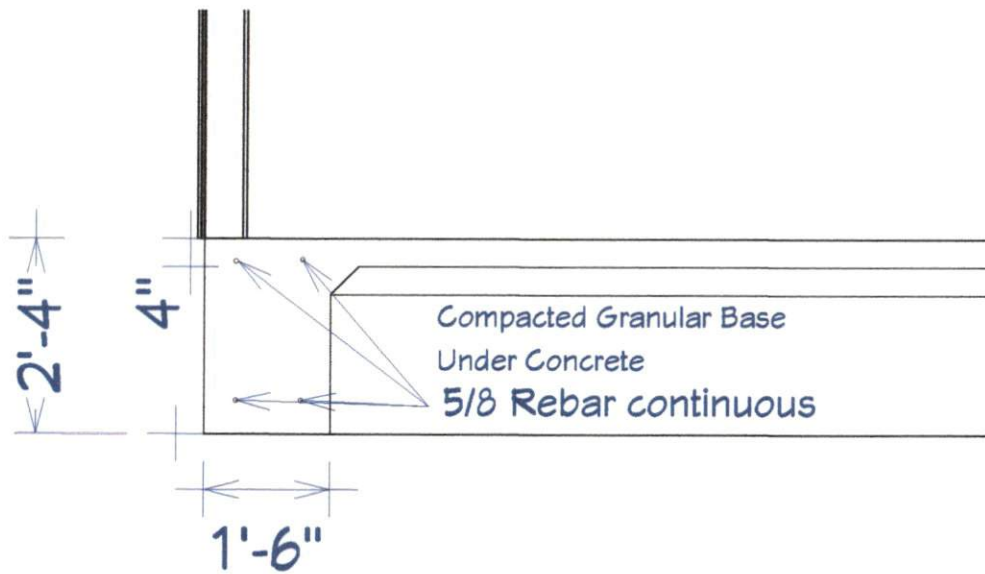
Cross Section 1
