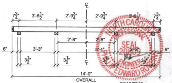
SECTION VIEW
