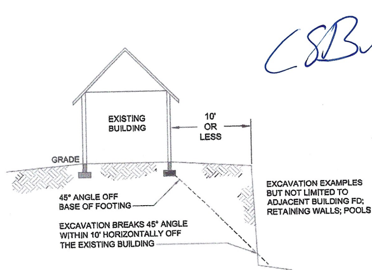
FIGURE R403.1.9 EXCAVATIONS NEAR FOOTINGS OR FOUNDATIONS
