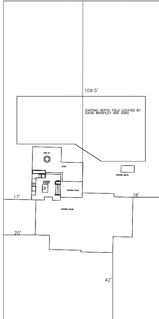
1 SITE PLAN 1" = 30'-0"
