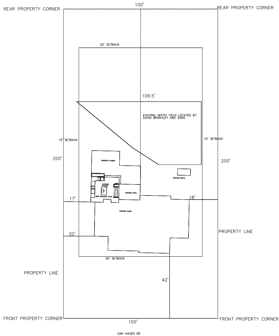
1 SITE PLAN 1" = 30'-0"
