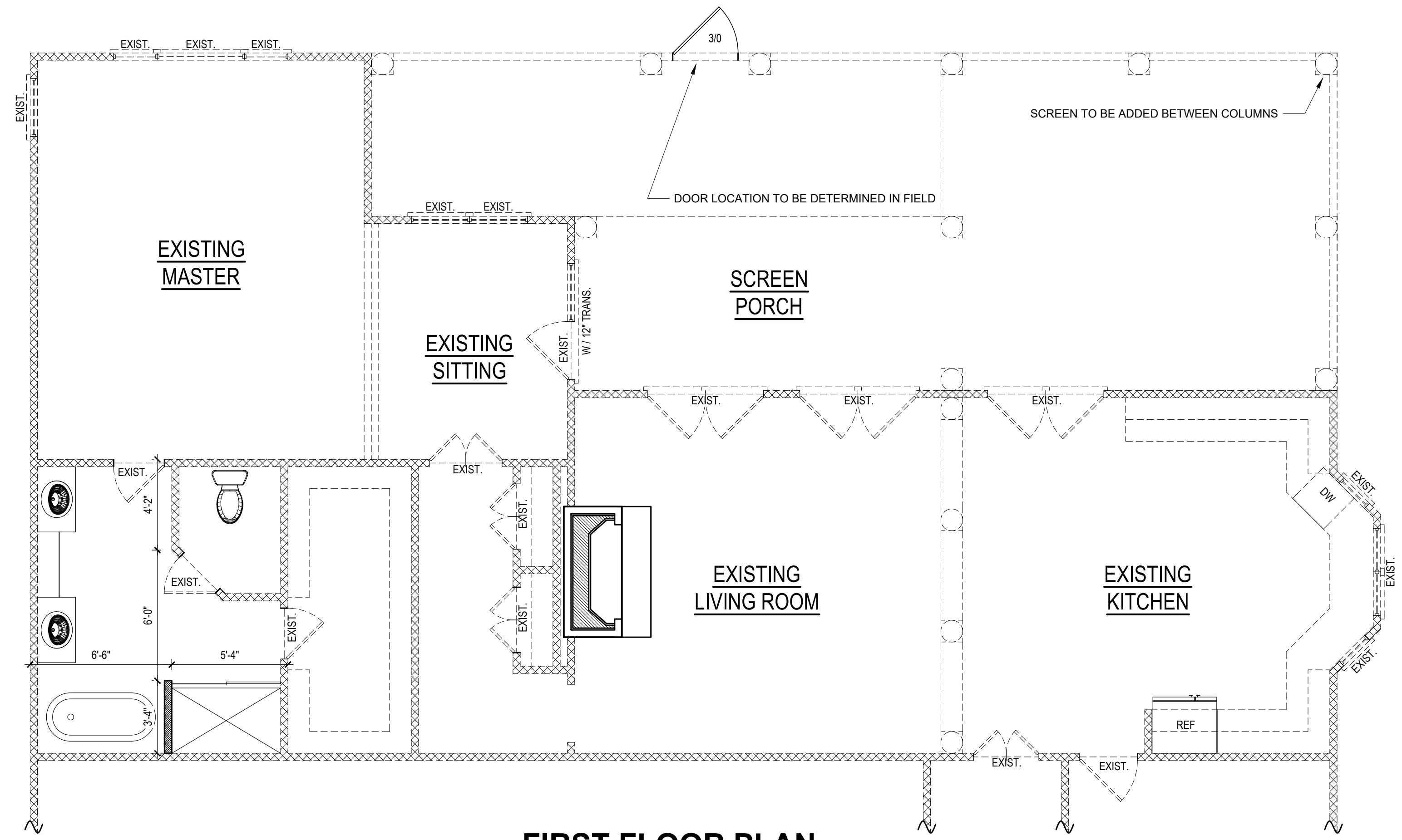
FIRST FLOOR PLAN 1/4" = 1'-0" CEILING HGT. = EXIST.
