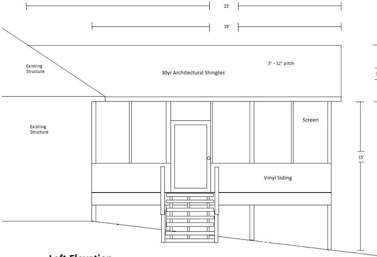
Left Elevation
