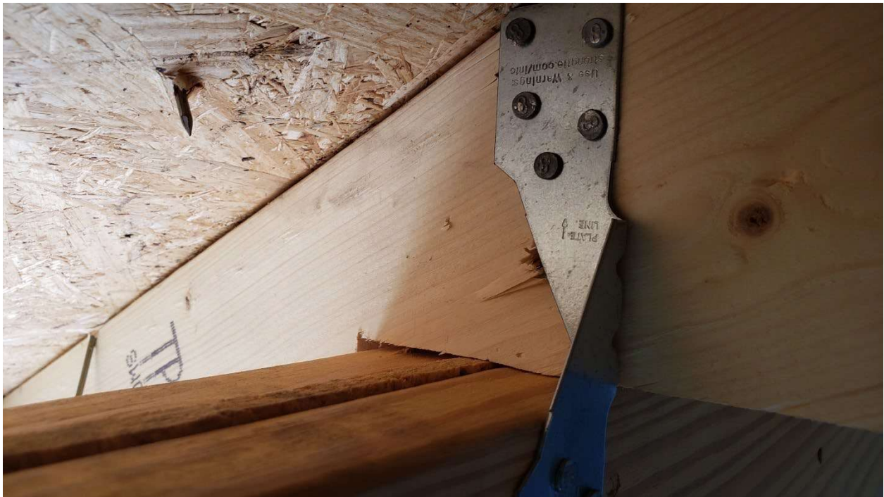
Example of notched rafters
