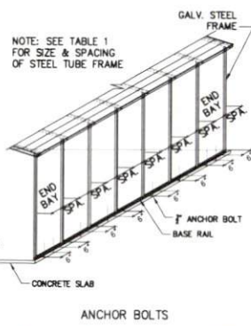
ANCHOR BOLTS
