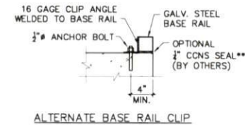
ALTERNATE BASE RAIL CLIP
