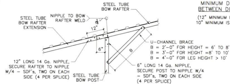
10 BOW/POST DETAIL
