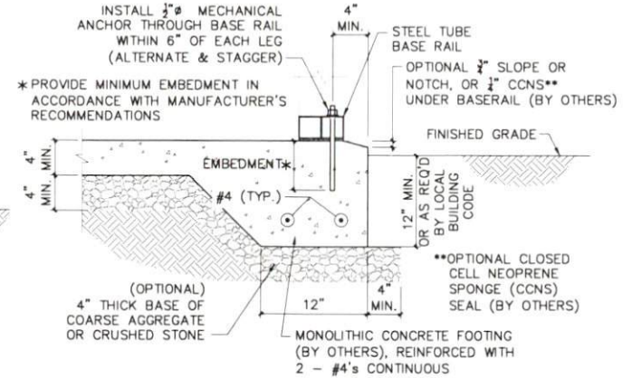
2 CONCRETE BASE RAIL ANCHORAGE (DOUBLE LEG)
