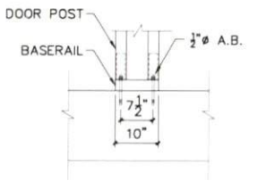
13 MINIMUM DISTANCE BETWEEN DOORWAYS
