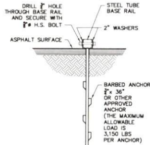
ASPHALT ANCHOR DETAIL
