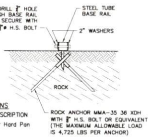
ROCK BASE RAIL ANCHOR DETAIL
