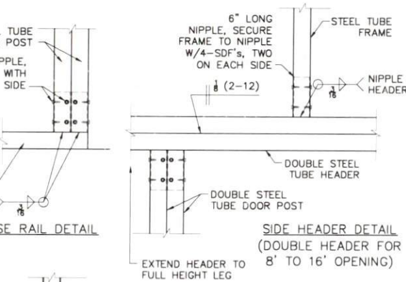
7 BOW / HEADER DETAIL
