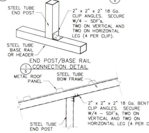
1 END POST/BASE RAIL CONNECTION DETAIL
