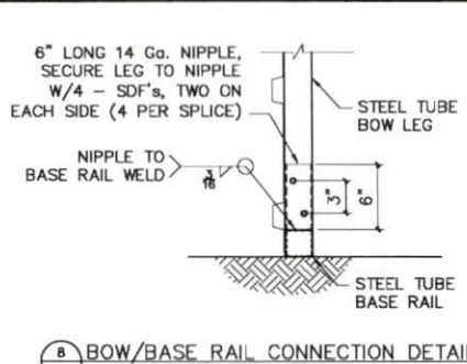
8 BOW/BASE RAIL CONNECTION DETAIL
