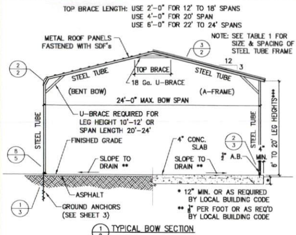
1 2 TYPICAL BOW SECTION
