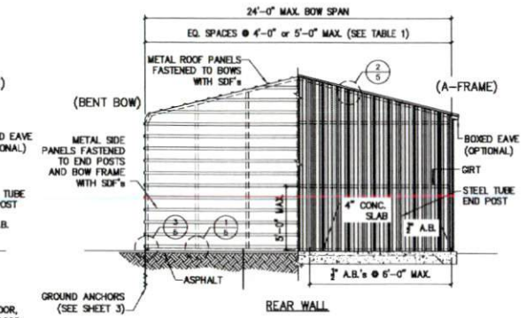
REAR WALL
