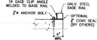
ALTERNATE BASE RAIL CLIP
