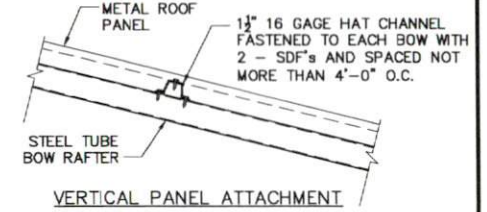
VERTICAL PANEL ATTACHMENT
