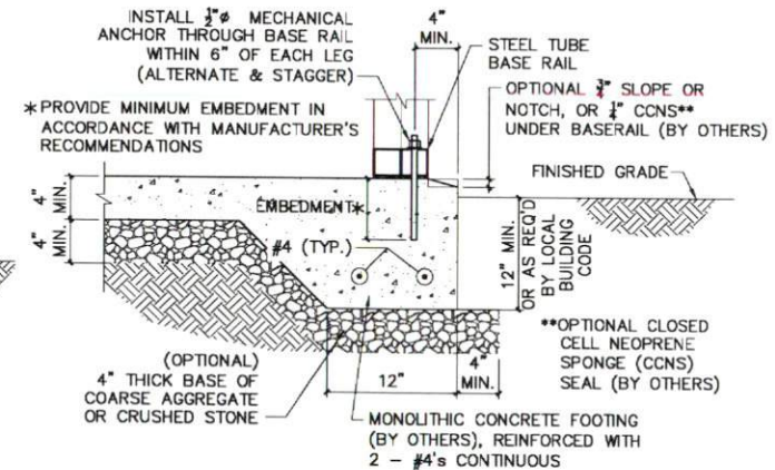
2 CONCRETE BASE RAIL ANCHORAGE (DOUBLE LEG) 3
