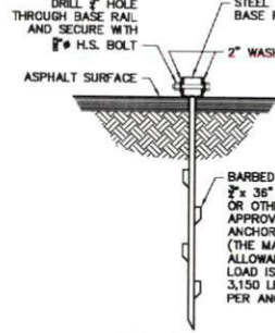
ASPHALT ANCHOR DETAIL
