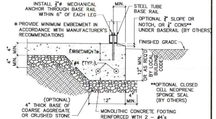
2 CONCRETE BASE RAIL ANCHORAGE (SINGLE LEG) 3
