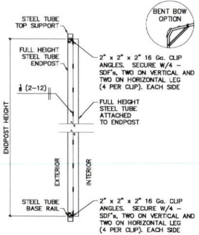
DOUBLE ENDPOST
