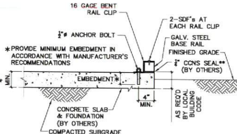
2 ALTERNATE BASE RAIL ANCHORAGE 3
