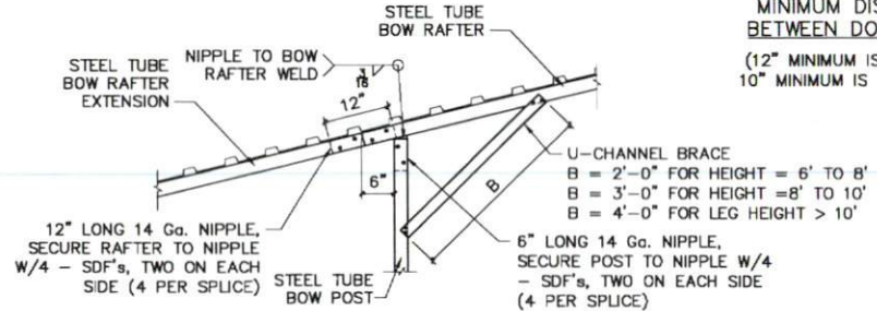
BOW/POST DETAIL
