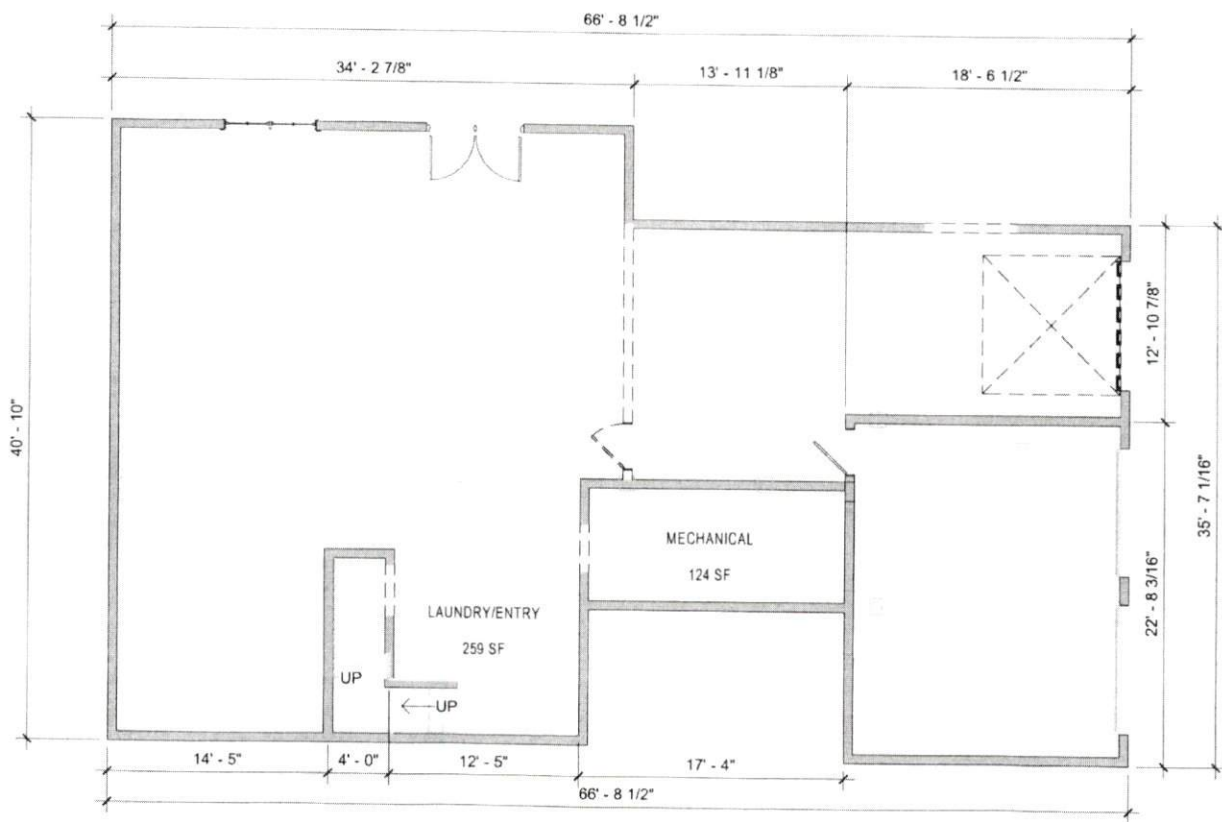
1 BASEMENT DEMOLITION PLAN
