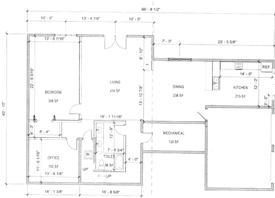
1 BASEMENT NEW CONSTRUCTION
