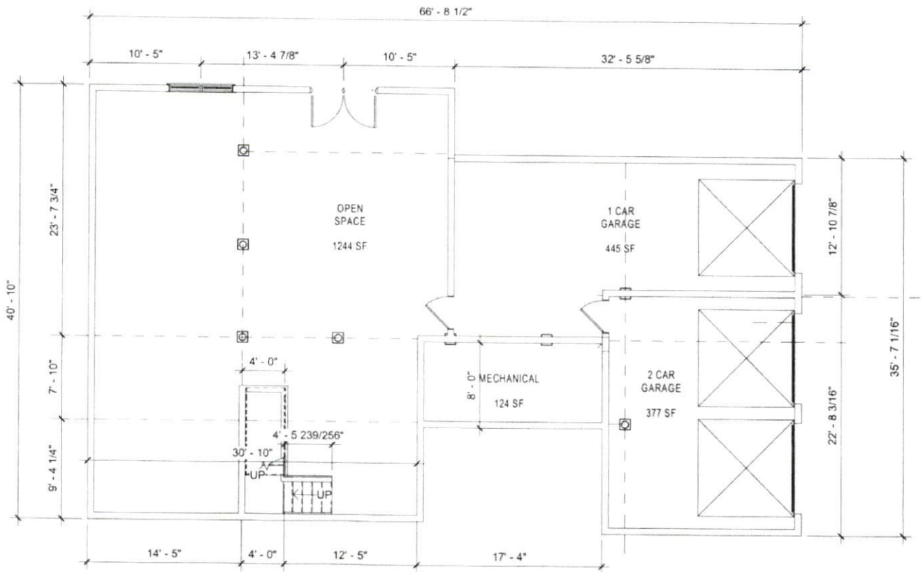
1 BASEMENT EXISTING PLAN
