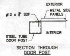
SECTION THROUGH ROLL-UP DOOR POST
