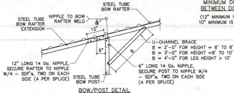
BOW/POST DETAIL
