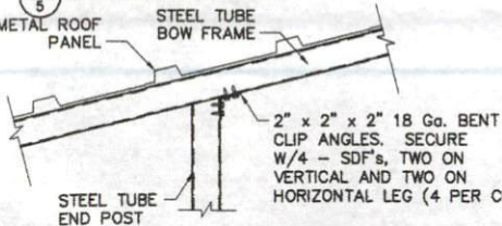
2 END POST TO BOW FRAME CONNECTION
