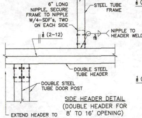
7 BOW / HEADER DETAIL
