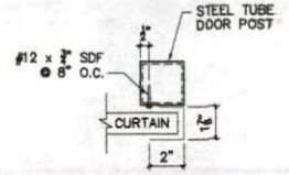
SECTION THROUGH ROLL-UP DOOR POST
