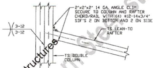
LEAN-TO RAFTER TO RAFTER COLUMN CONNECTION DETAIL FOR RAFTER SPANS ≤ 12'-0"
