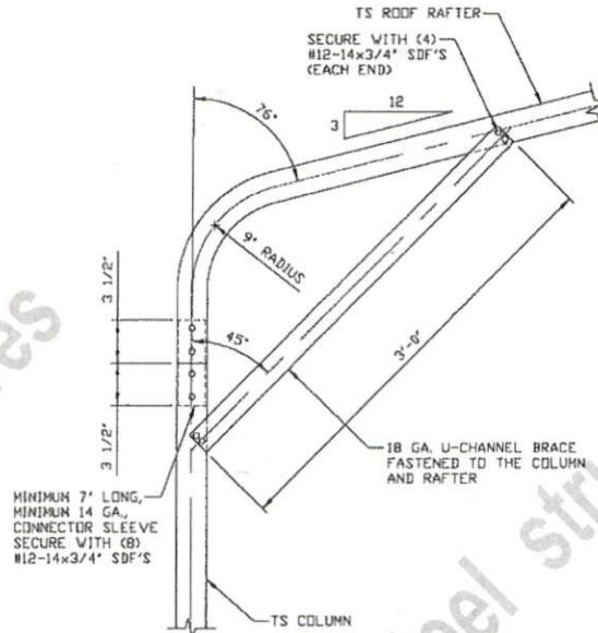
BOW EAVE RAFTER/CORNER POST CONNECTION DETAIL FOR HEIGHTS 8'-0" < TO <= 10'-0" SCALE: NTS
