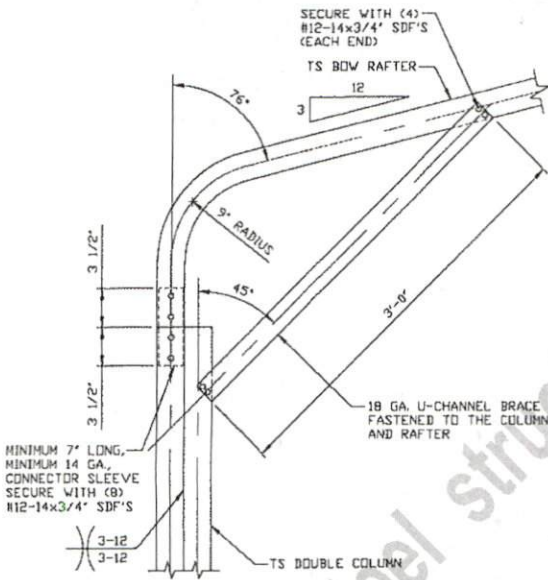
BOW EAVE RAFTER/CORNER POST CONNECTION DETAIL FOR HEIGHTS 10'-0" < TO <= 16'-0" SCALE: NTS
