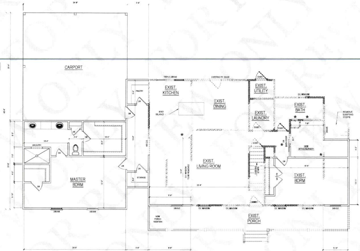
FIRST FLOOR PLAN 1/4" = 1'-0" CEILING HGT. = 9'-0"
