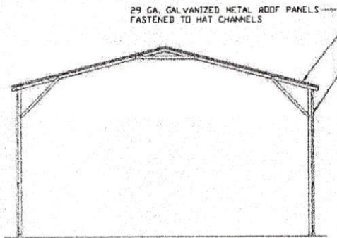
TYPICAL SECTION VERTICAL ROOF OPTION SCALE: NTS
