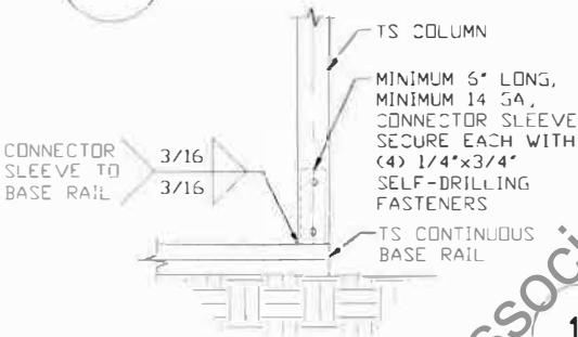
10A COLUMN/BASE RAIL CONNECTION DETAIL SCALE: NTS
