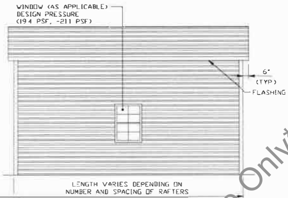
TYPICAL SIDE ELEVATION-HORIZONTAL ROOF
