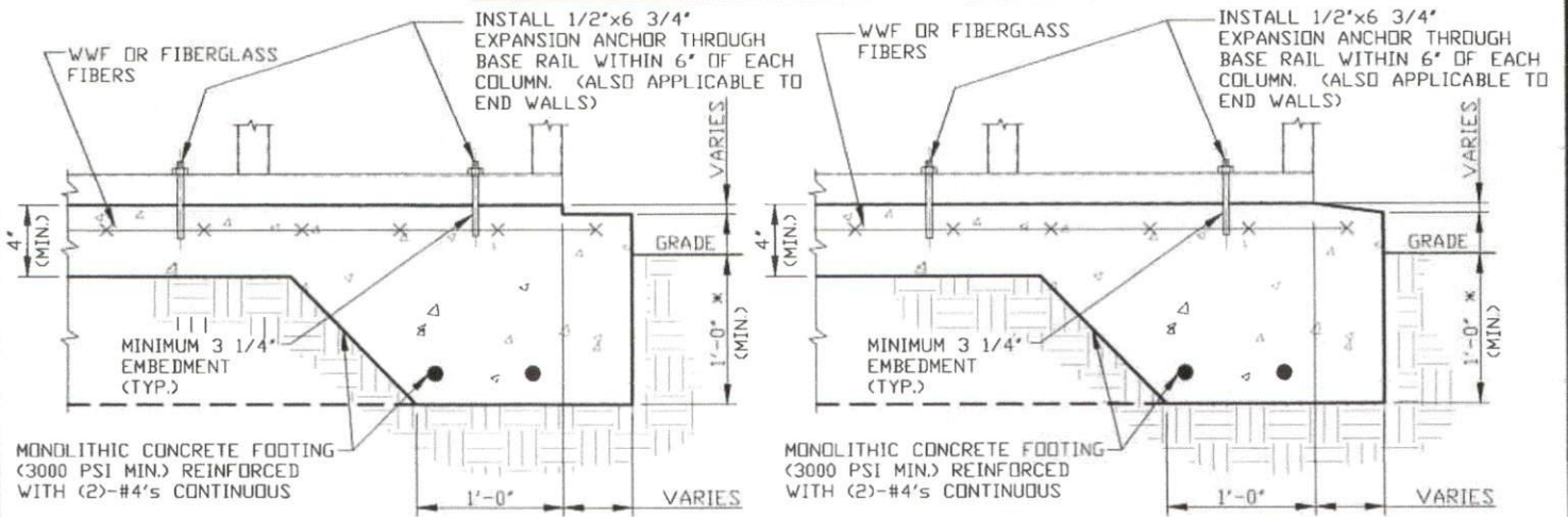
2A CONCRETE MONOLITHIC SLAB BASE RAIL ANCHORAGE SCALE: NTS MINIMUM ANCHOR EDGE DISTANCE IS 4". * COORDINATE WITH LOCAL BUILDING CODE AND/OR D REGARDING MINIMUM FROST DEPTH (LENGTH).
