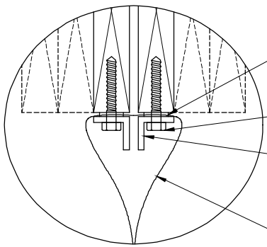
TIE-DOWN BRACKETS
